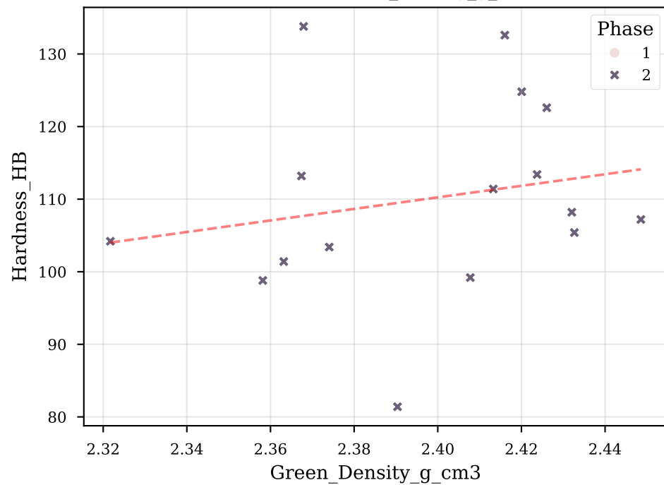
Hardness vs Green_Density_g_cm3
