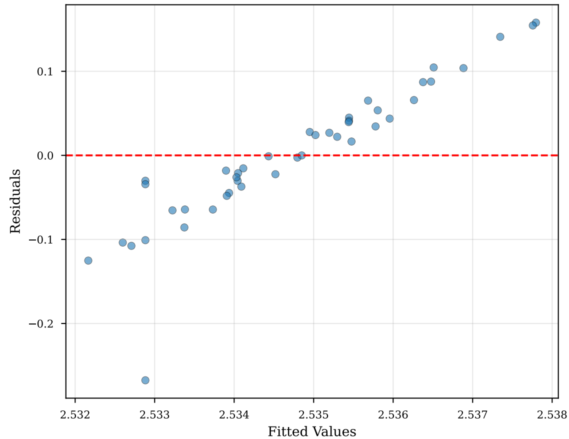
Density: Residuals vs Fitted
