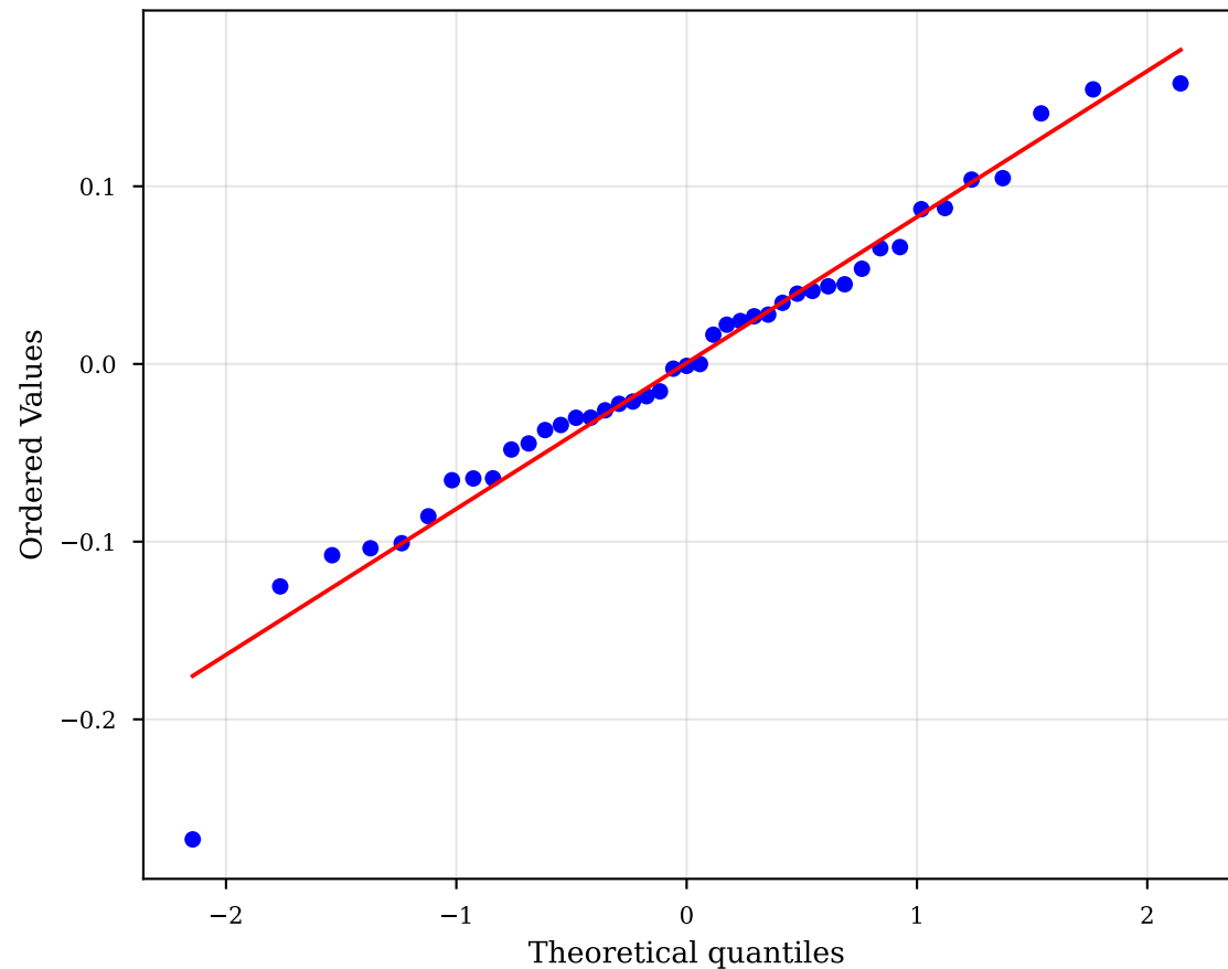
Density: Q-Q Plot
