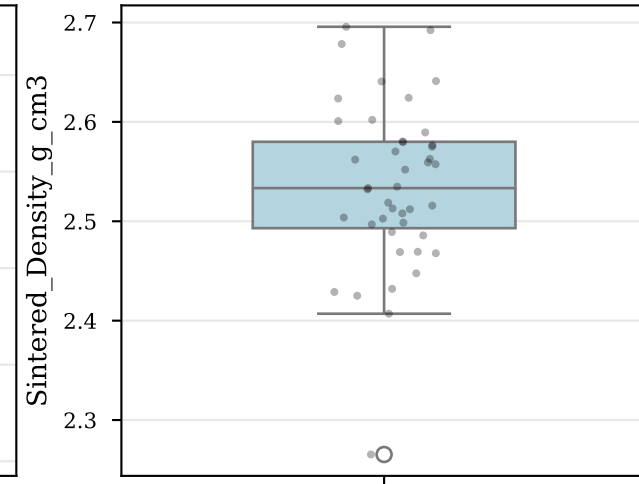
Sintered_Density_g_cm3
