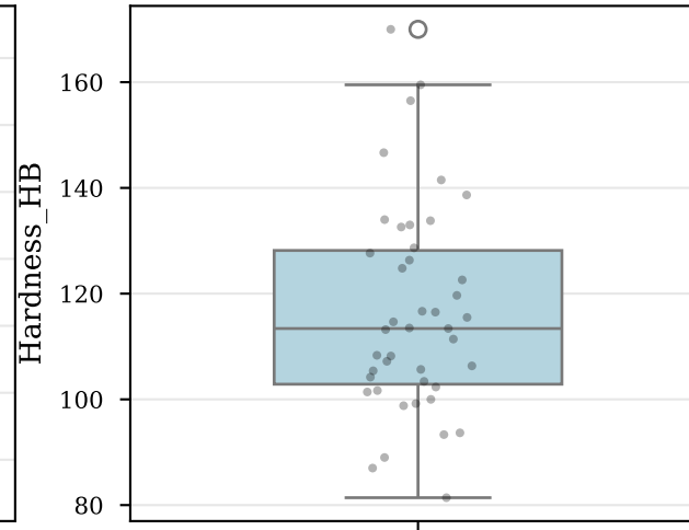
Hardness_HB
