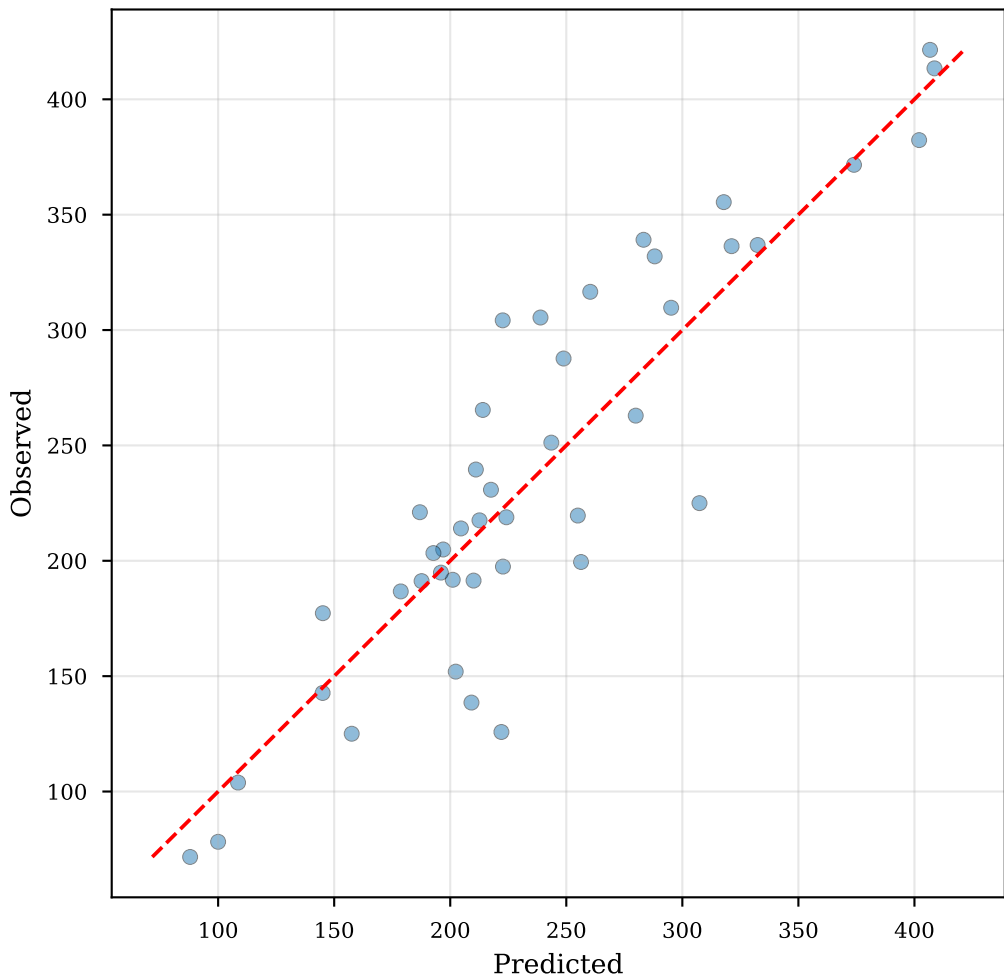
Calibration: Strength
