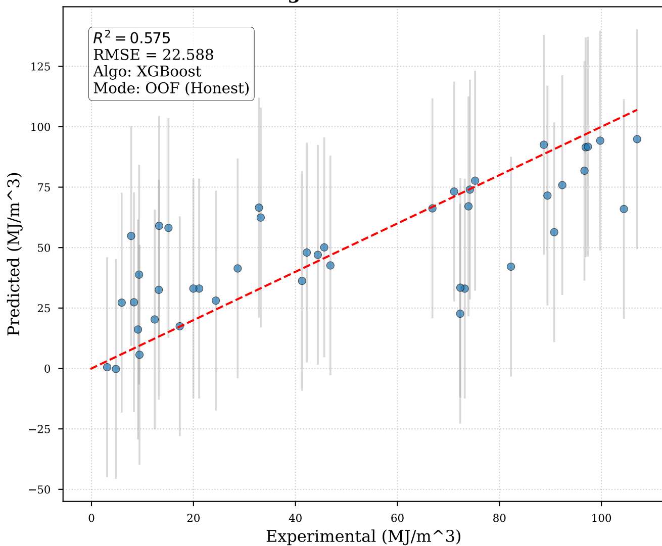
Toughness Prediction
