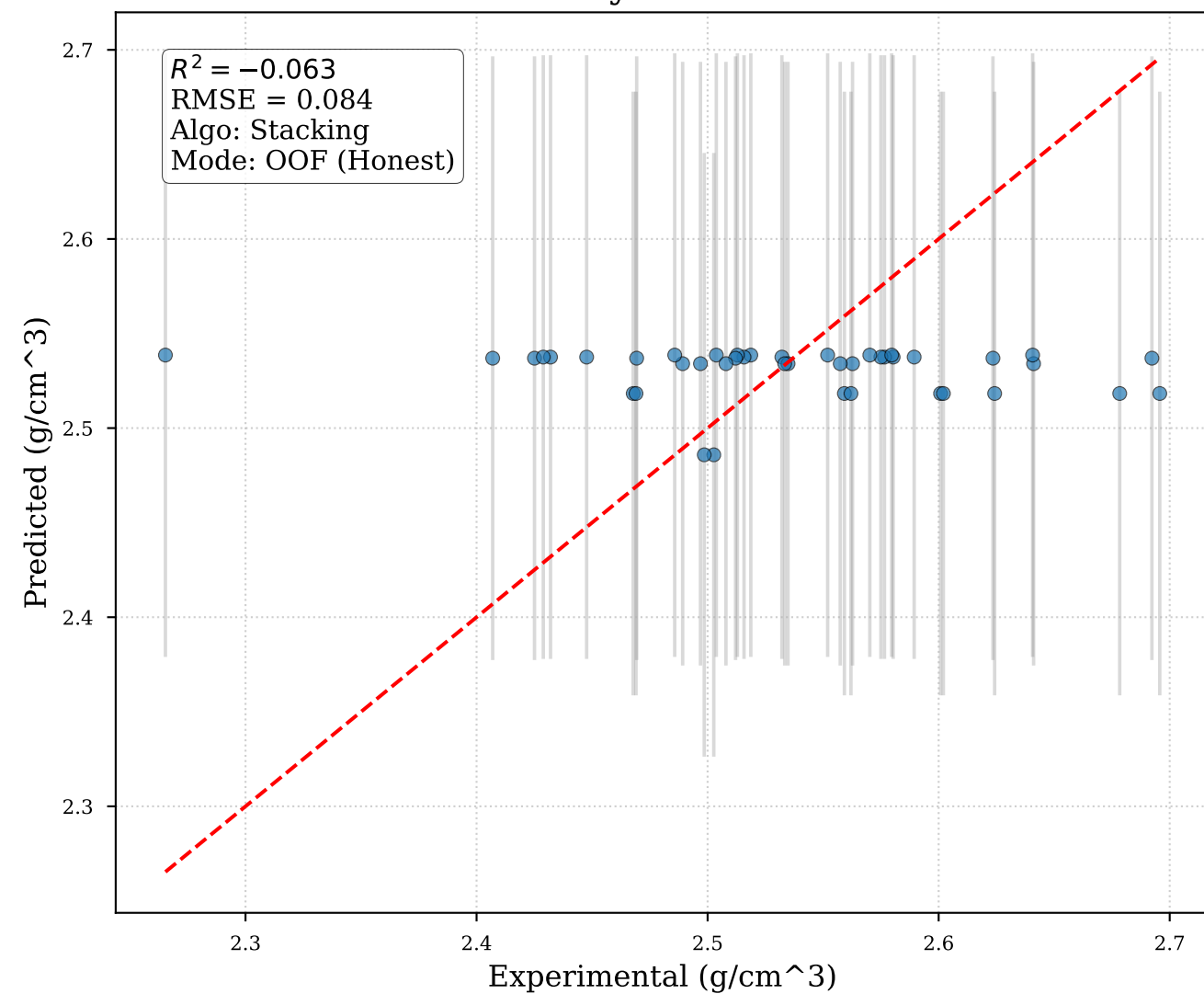
Density Prediction
