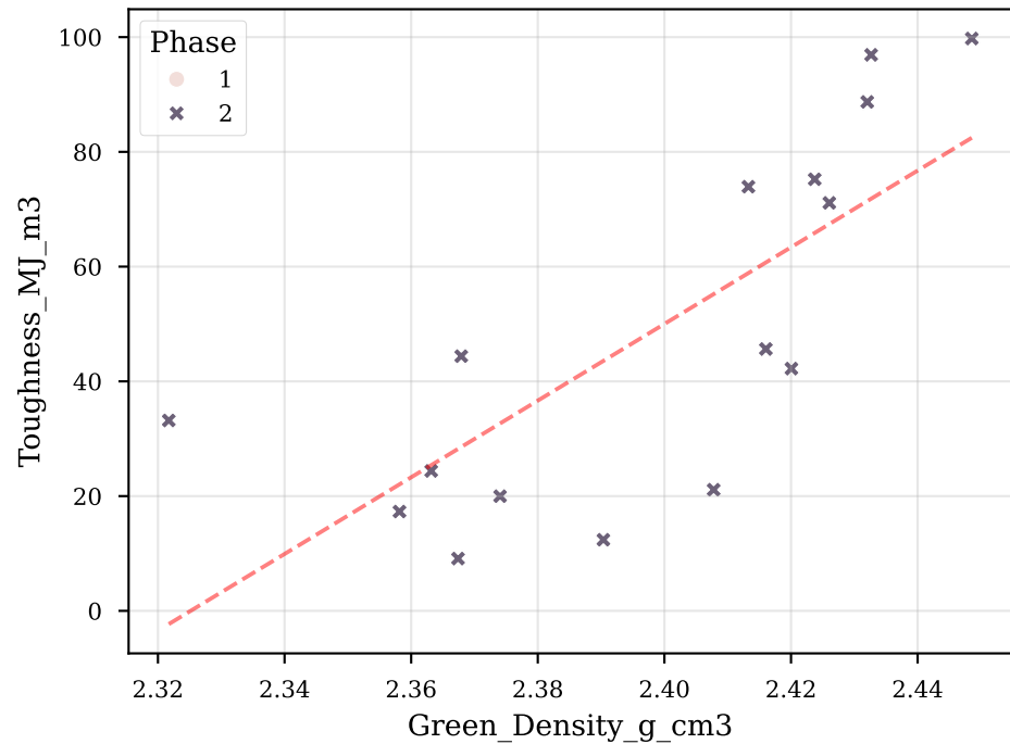
Toughness vs Green_Density_g_cm3
