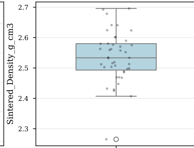
Sintered_Density_g_cm3
