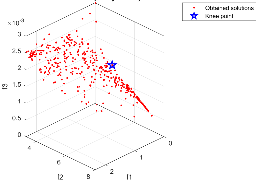
Pareto Front (3 Objectives)
