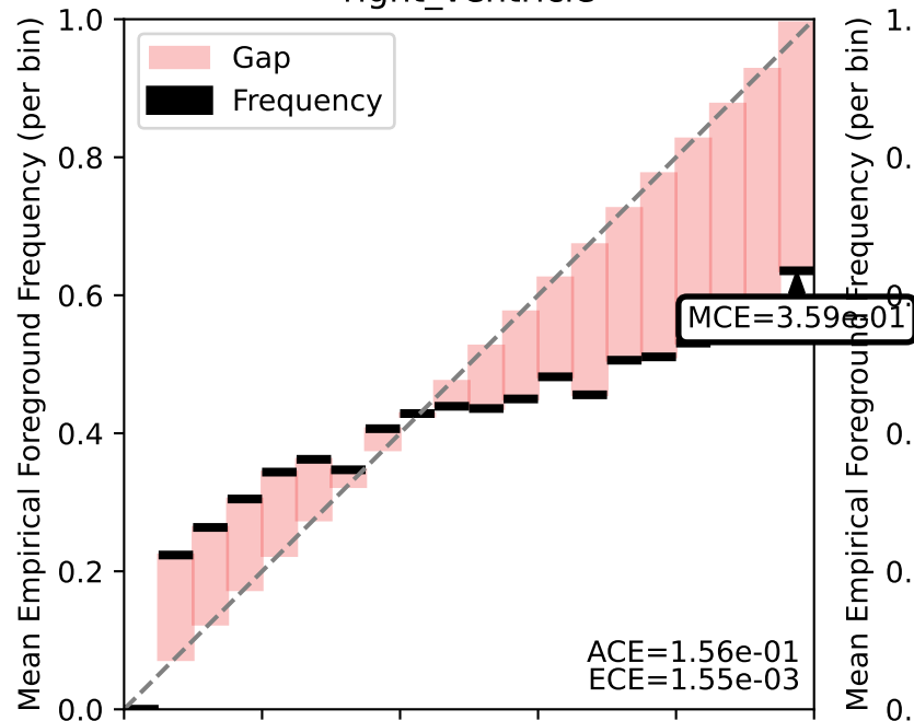
right_ventricle
