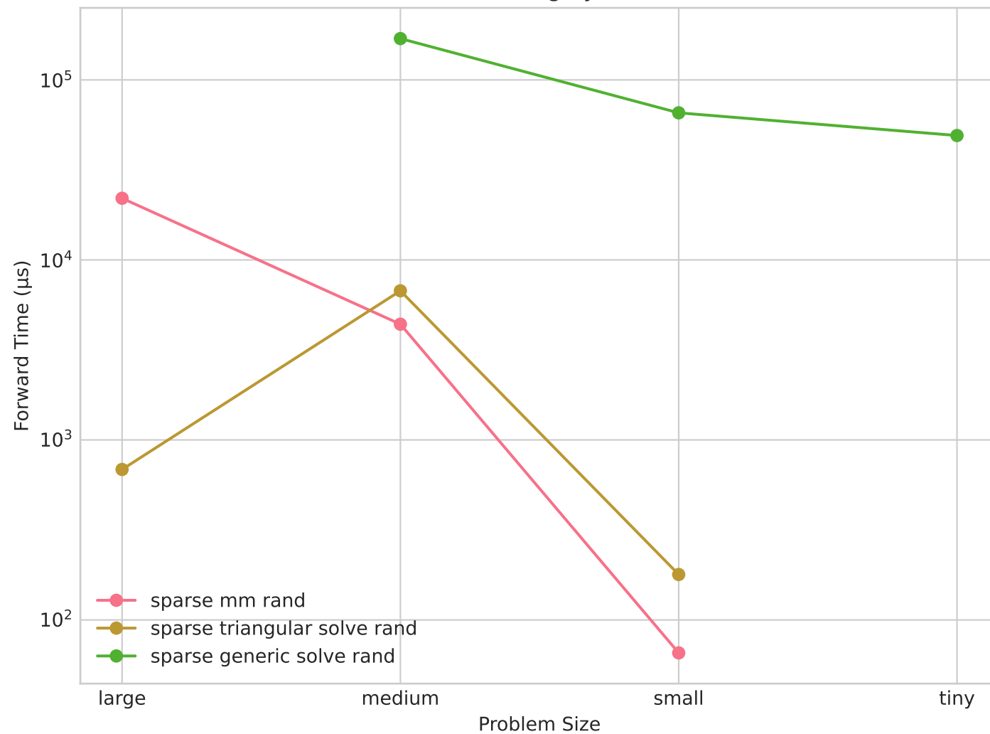
Performance Scaling by Problem Size
