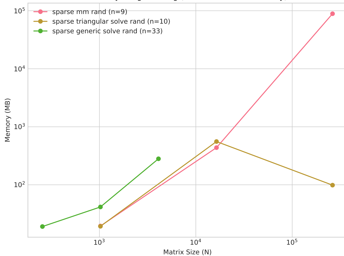
Memory Usage Scaling (Valid Measurements Only)
