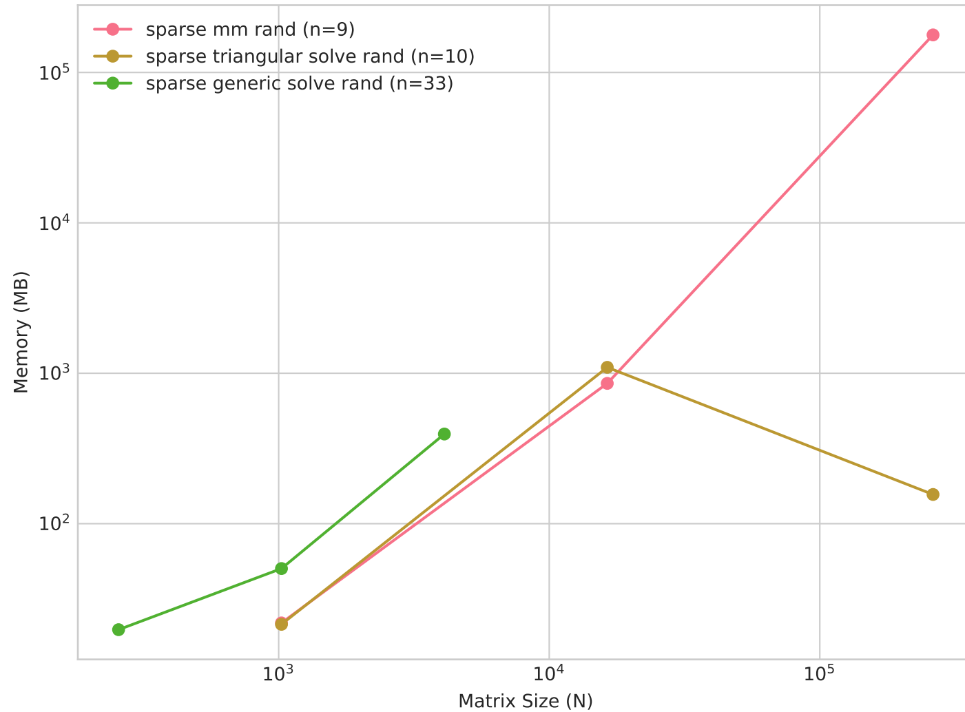
Memory Usage Scaling (Valid Measurements Only)
