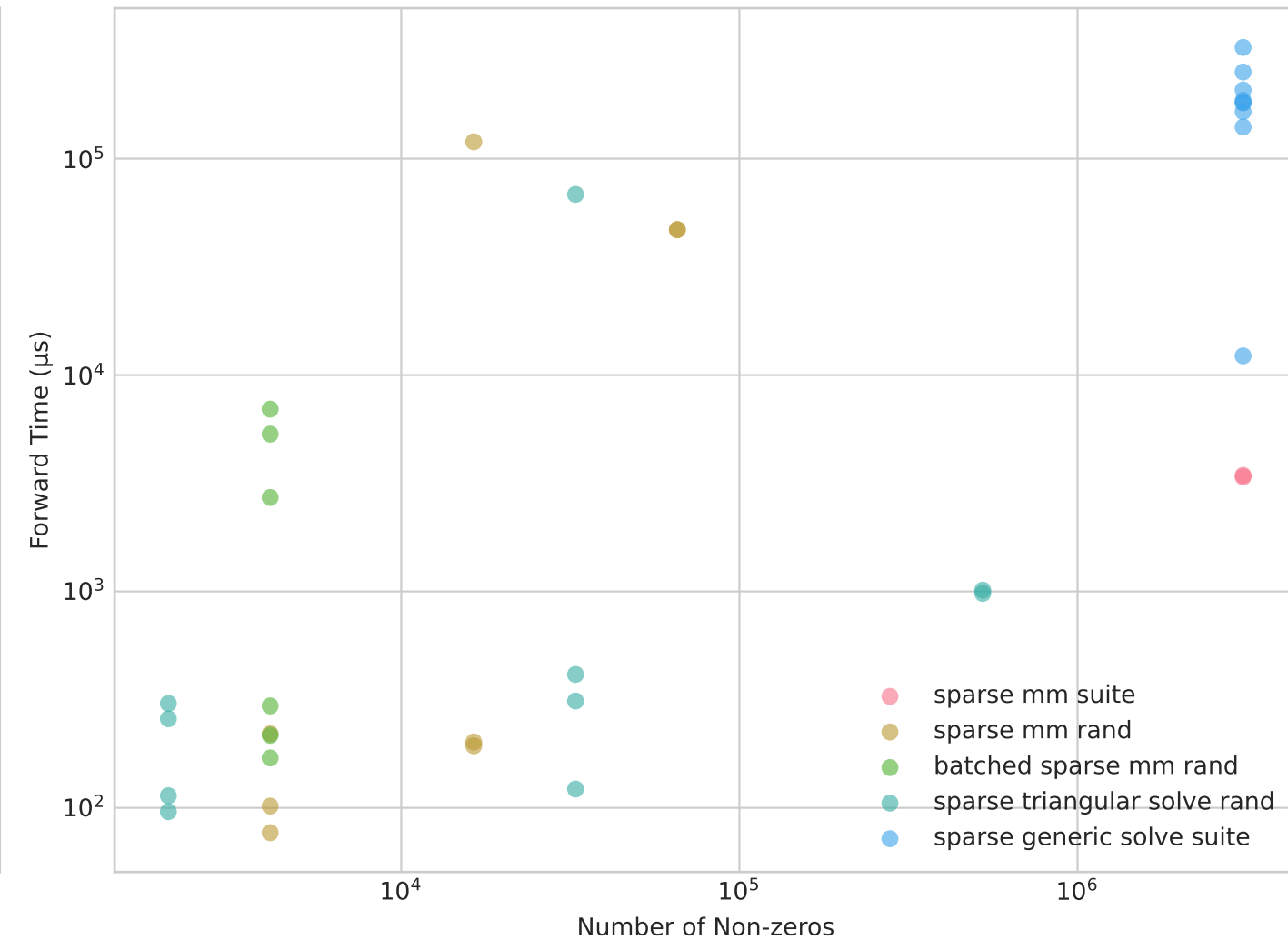
Performance vs Number of Non-zeros
