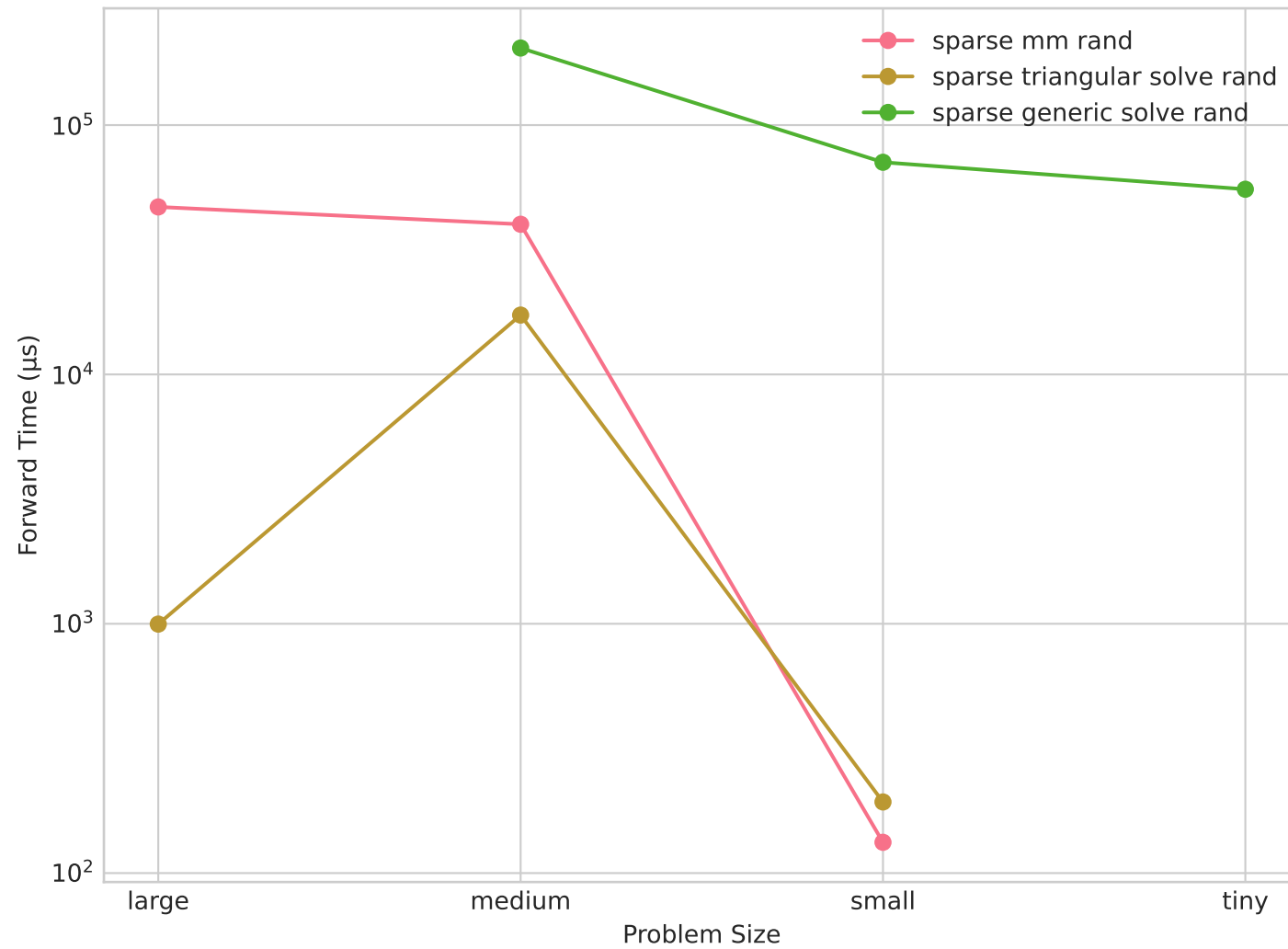
Performance Scaling by Problem Size
