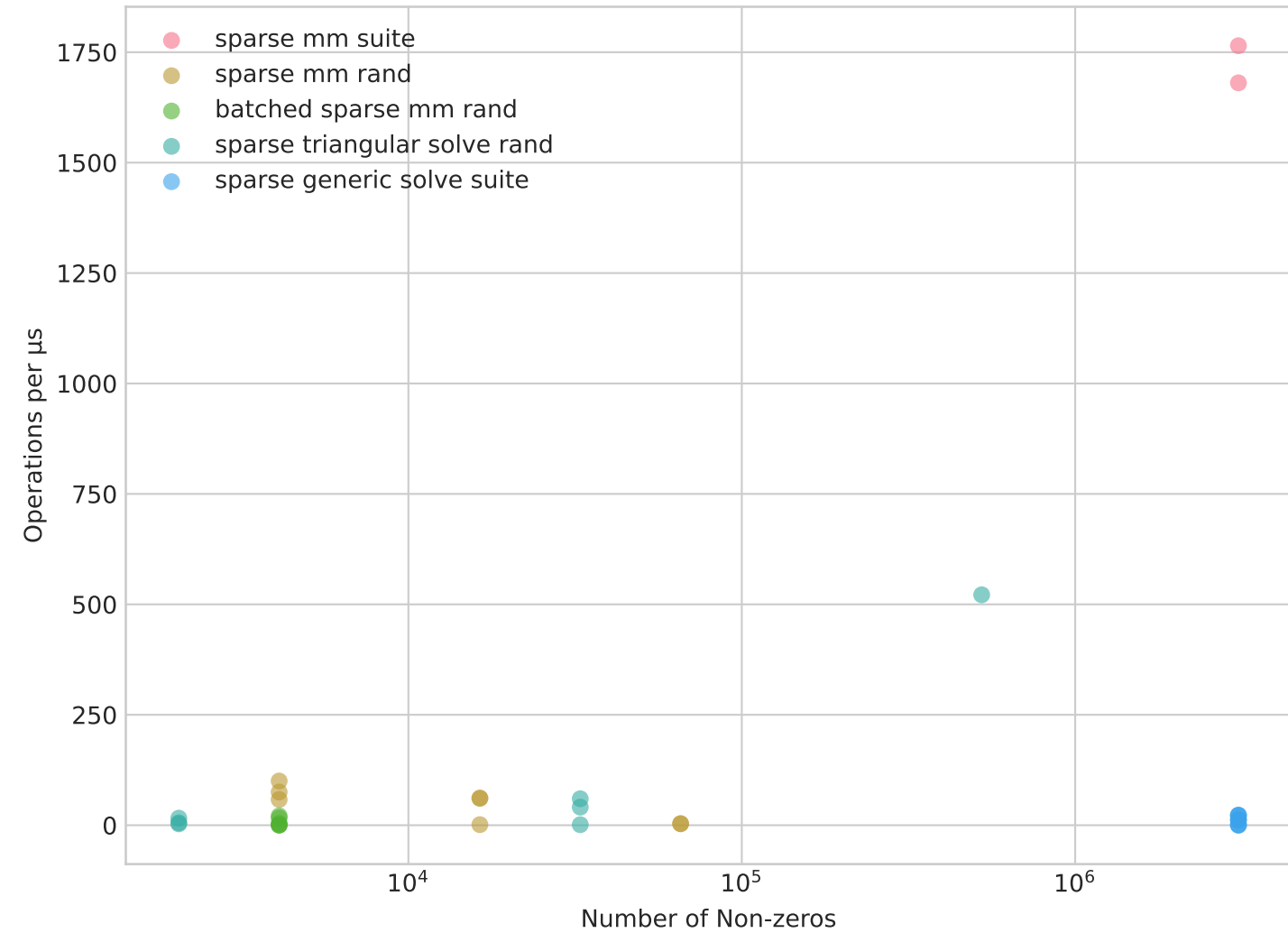
Computational Efficiency
