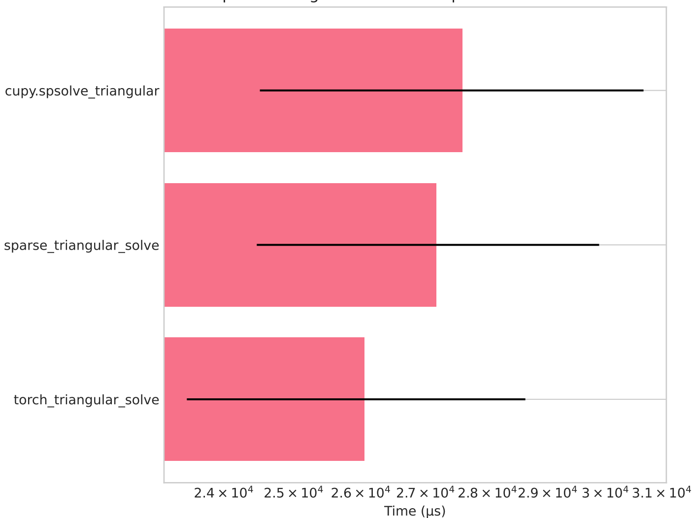
Sparse Generic Solve Suite - Forward Time
