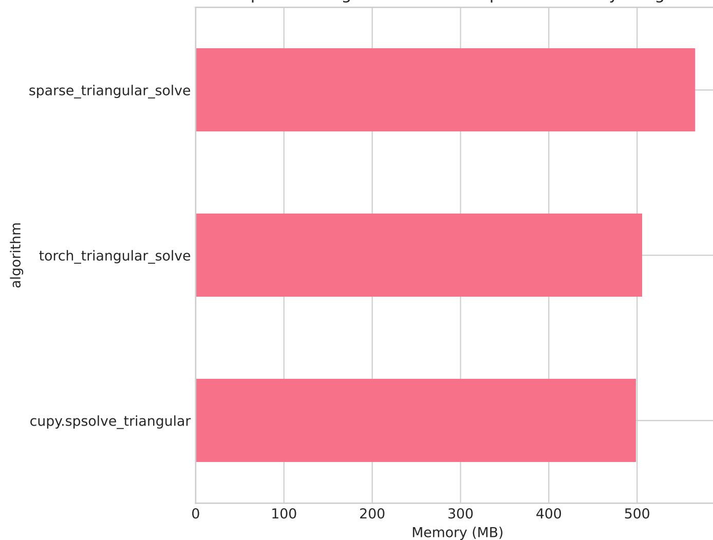
Sparse Generic Solve Suite - Memory Usage
