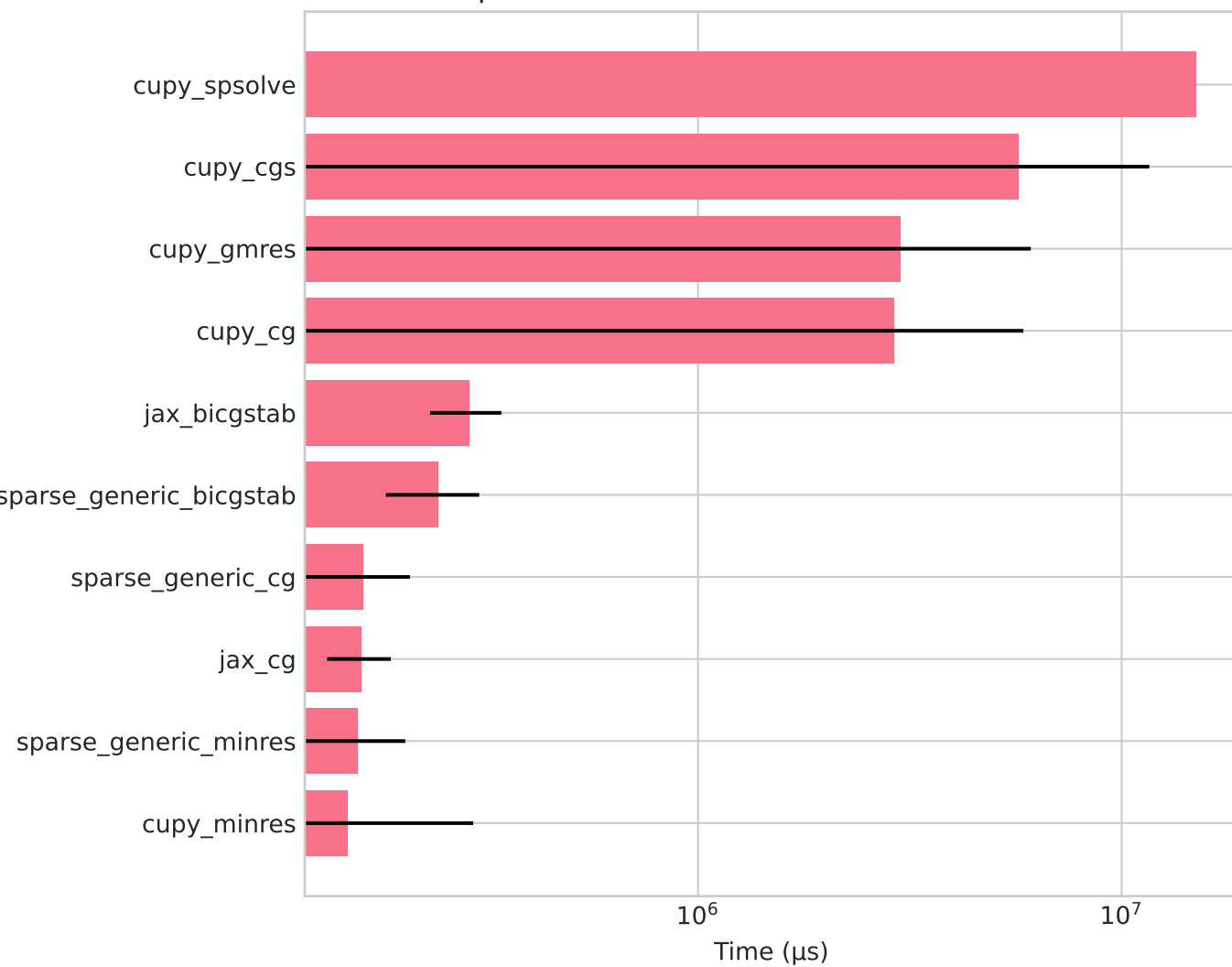
Sparse Generic Solve Suite - Forward Time
