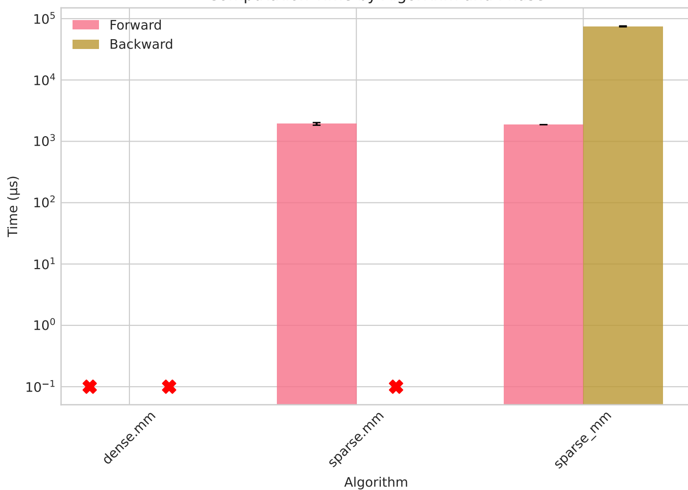
Computation Time by Algorithm and Phase
