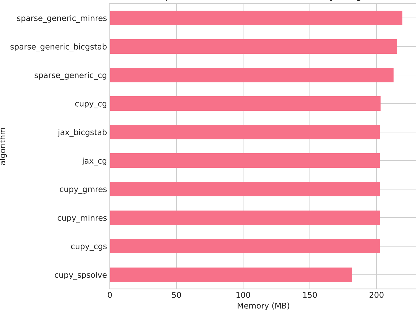
Sparse Generic Solve Suite - Memory Usage
