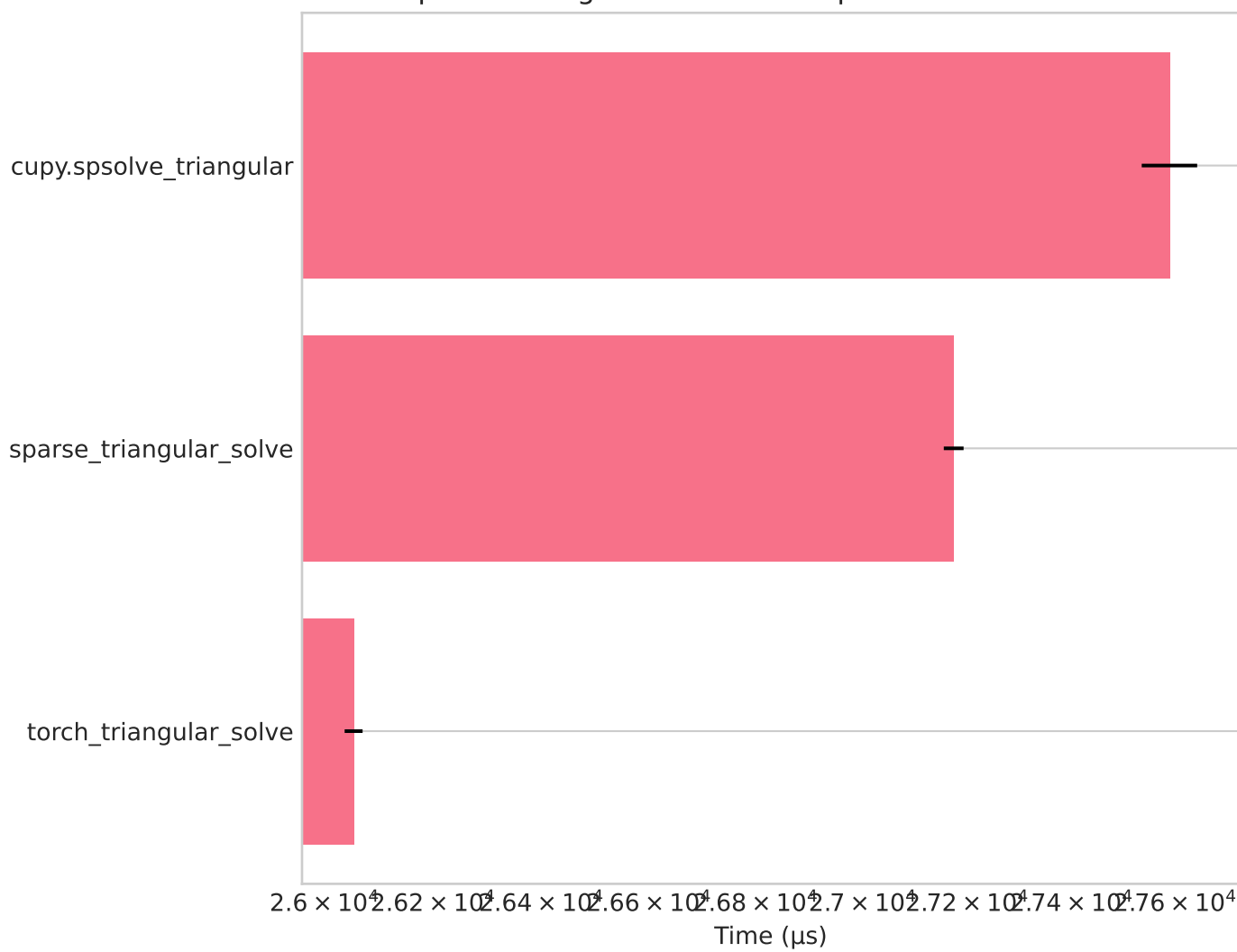
Sparse Generic Solve Suite - Forward Time
