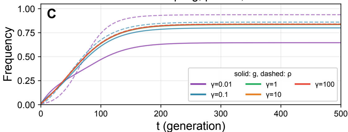
Dual-state coupling, \mu=0.01 , s=0.05
