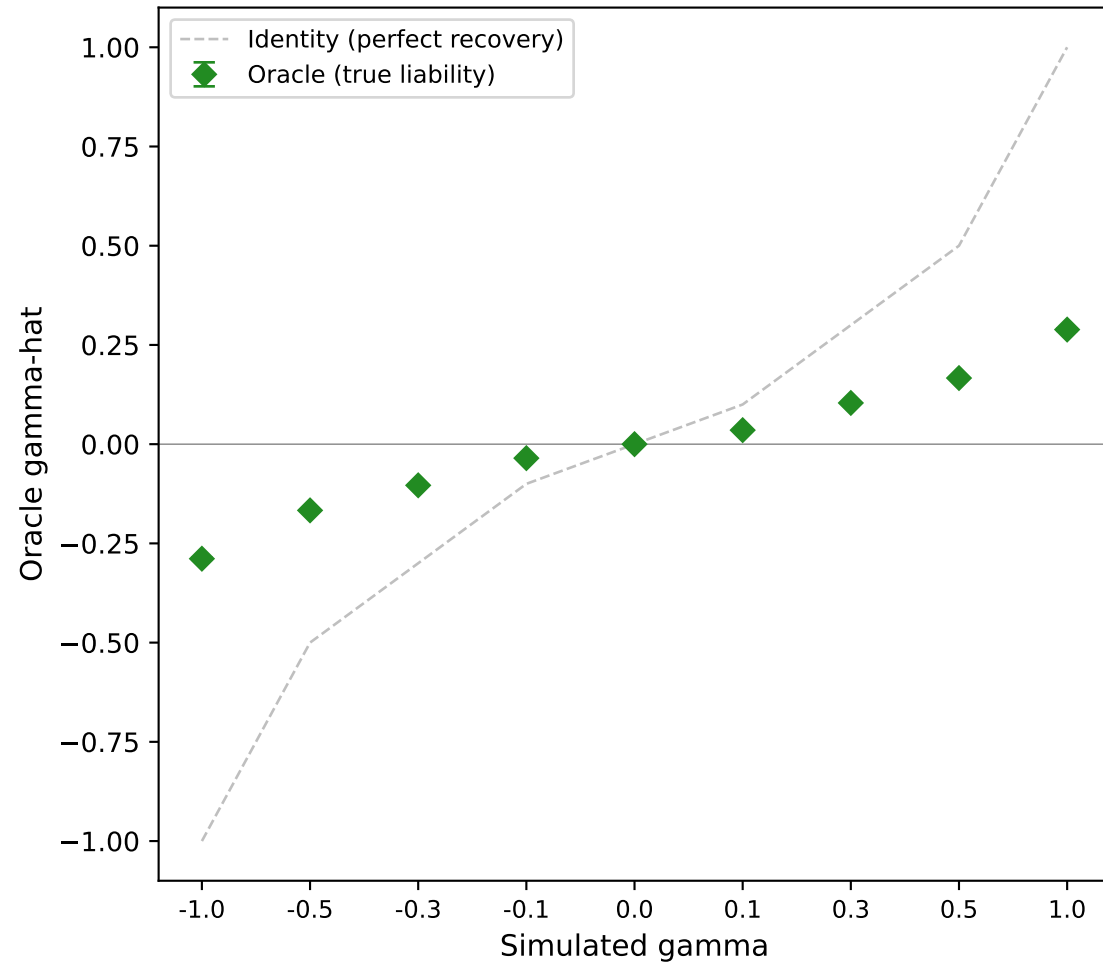
A. Oracle gamma recovery
