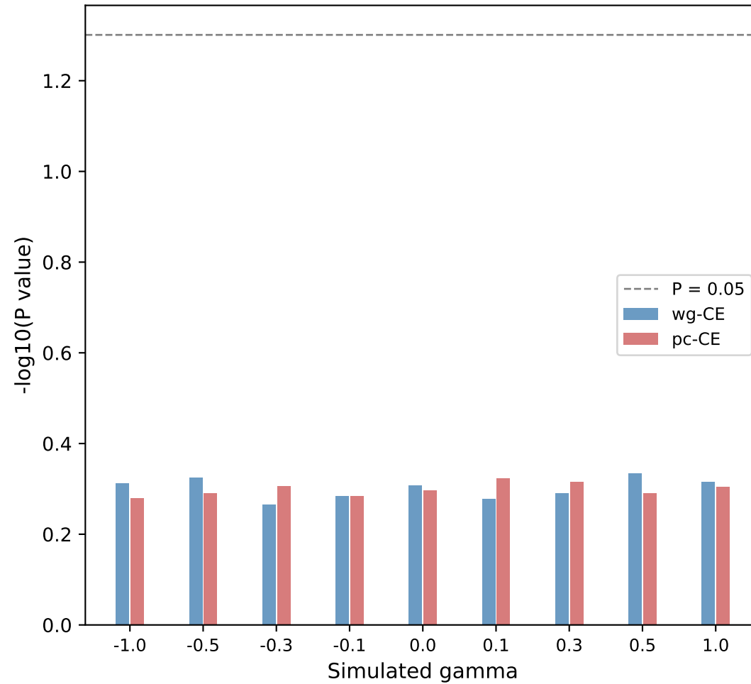
B. Significance (clumped PRS)
