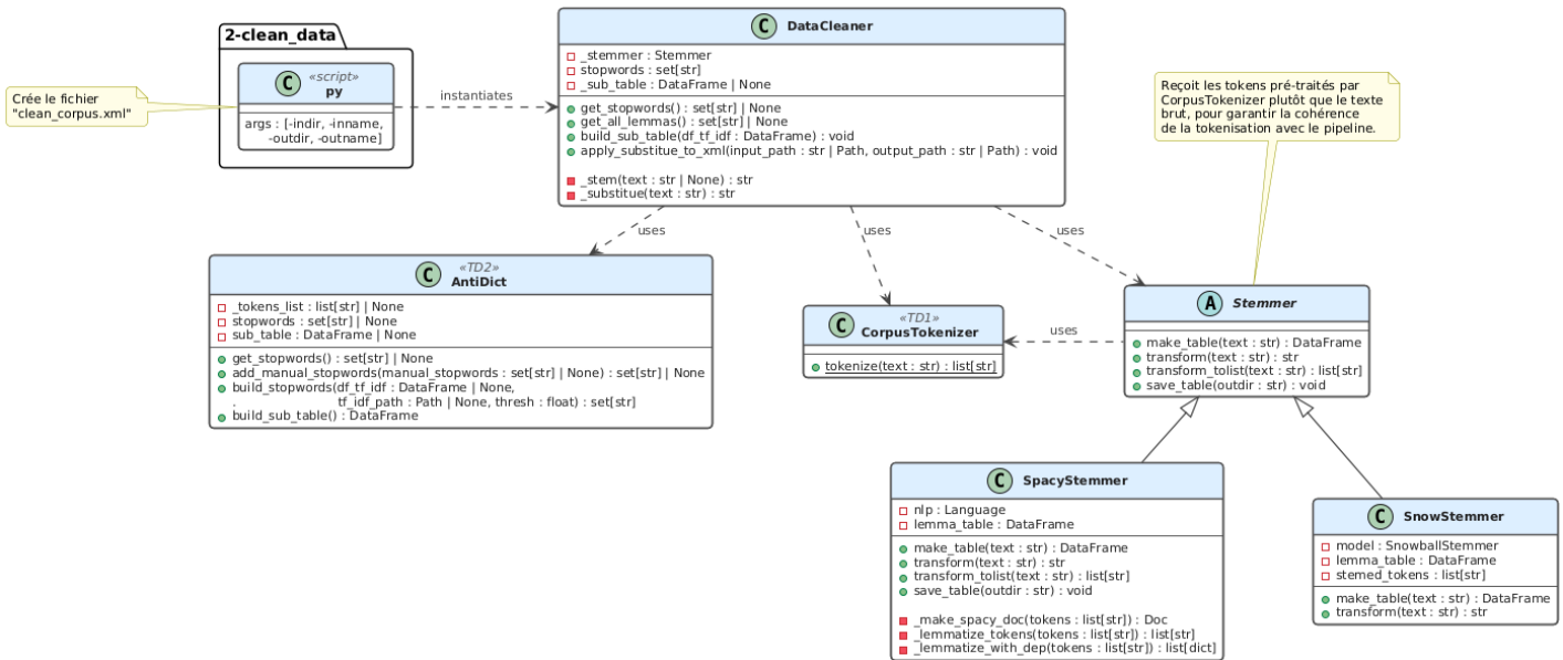
FIGURE 3.1 – UML Stemmer + AntiDict (TD1)
