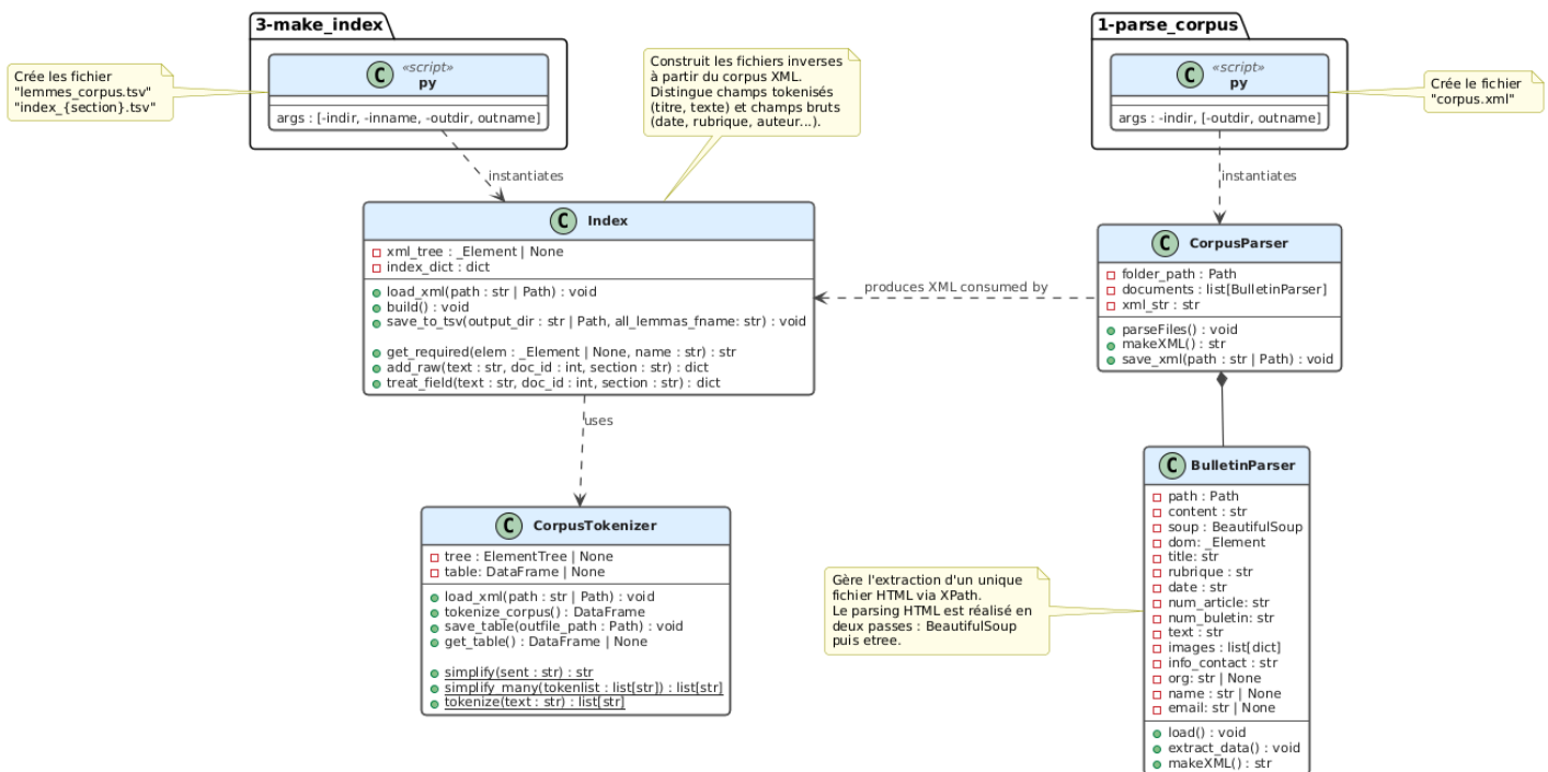
FIGURE 1.1 – UML Indexation (TD1)
