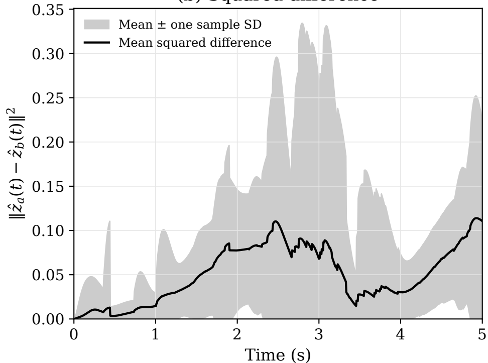
(b) Squared difference
