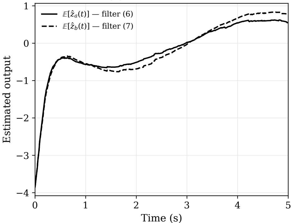
(a) Filter estimates
