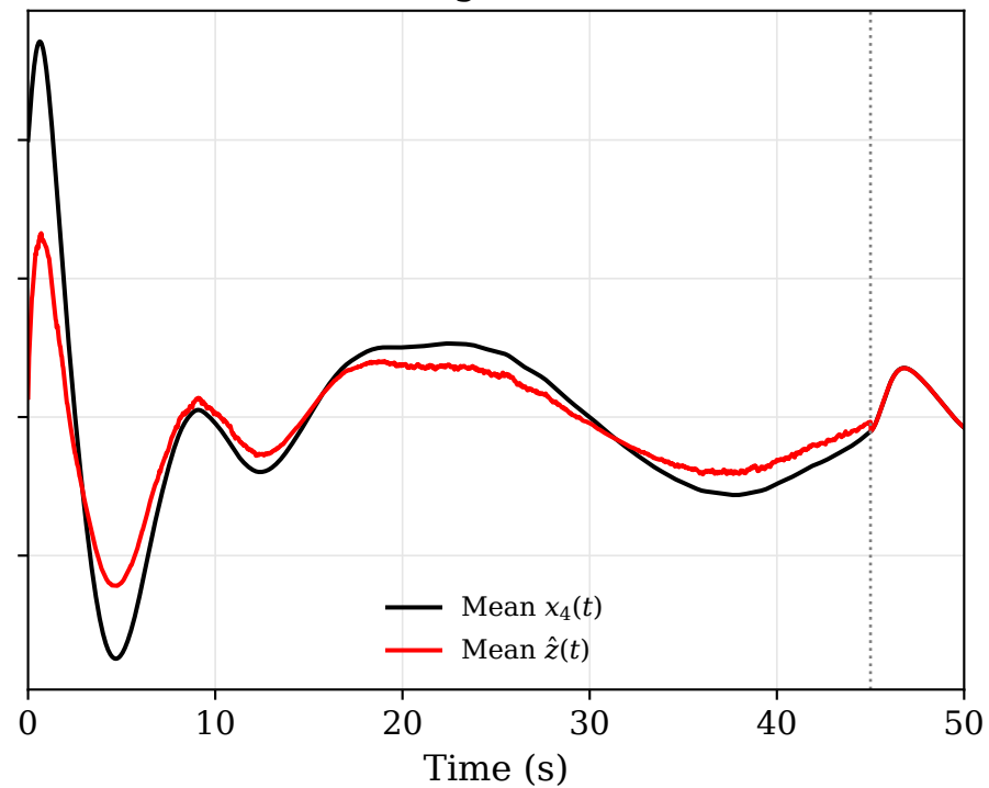
(b) Algorithm 1
