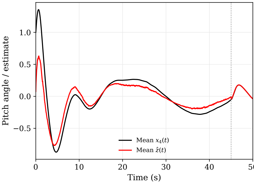
(a) Theorem 1
