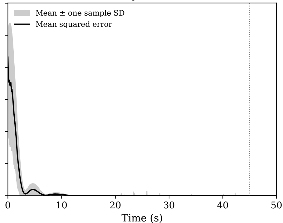
(b) Algorithm 1
