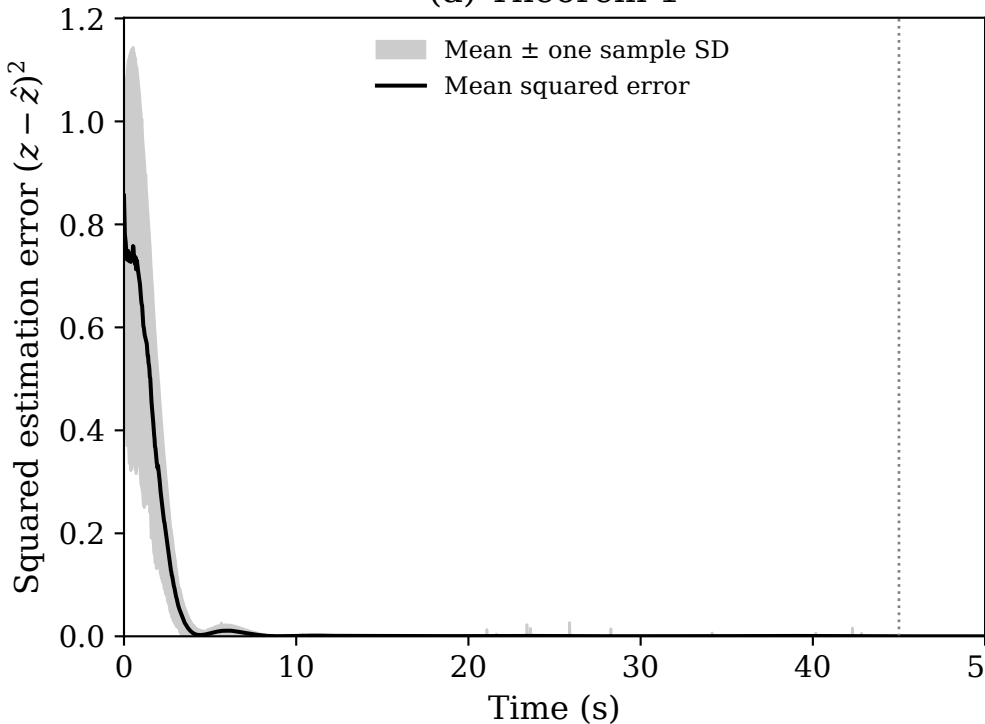
(a) Theorem 1
