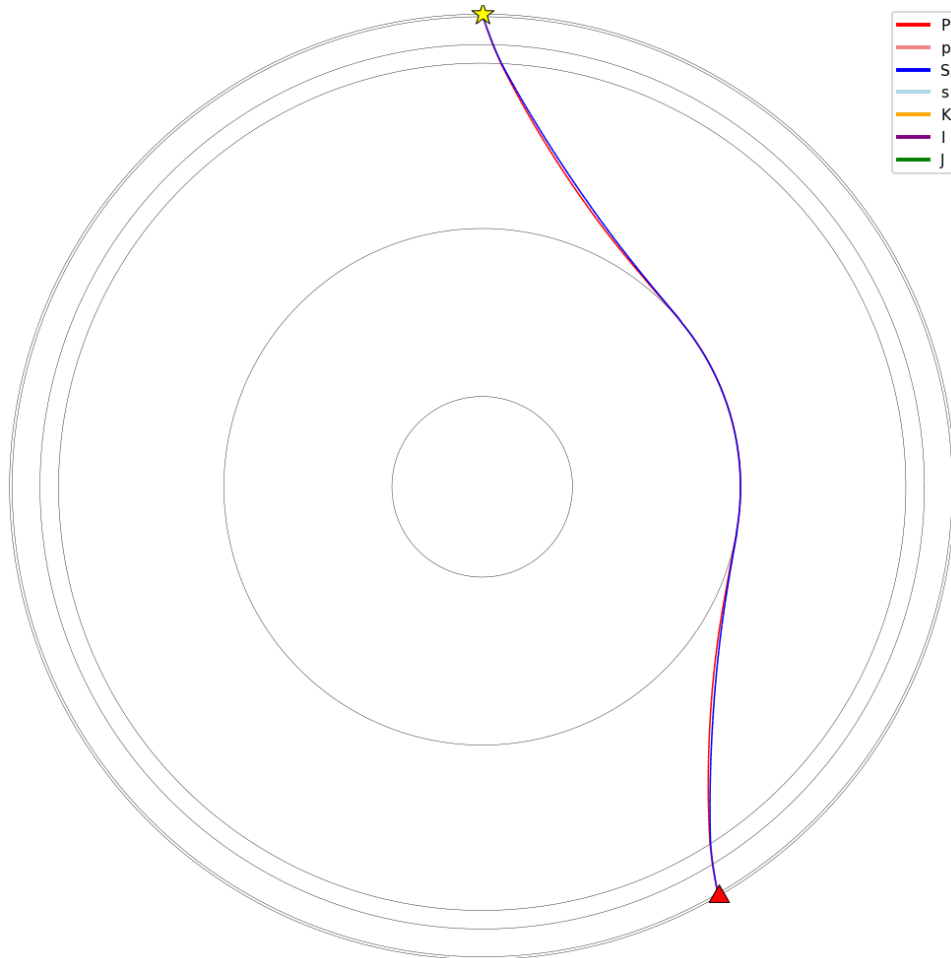
Figure 3: Ray paths for diffracted Pdif (red) and Sdif (blue) phases at an epicentral distance of 150^\circ , showing waves grazing along the Core-Mantle Boundary (CMB) in the Earth's cross-section.
