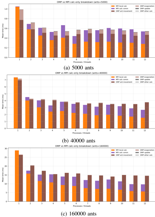
Fig. 5. MPI subdomain vs OpenMP computation-only breakdown for selected colony sizes.
