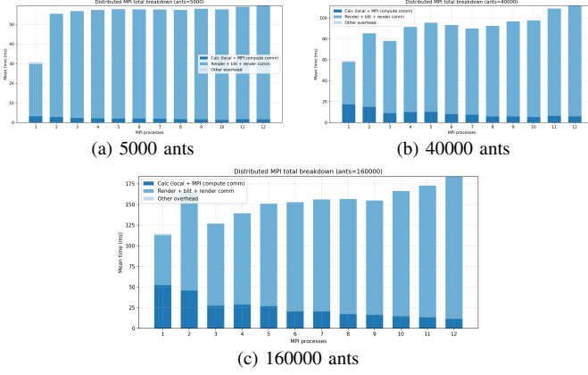
Fig. 2. MPI subdomain total iteration-time breakdown for selected colony sizes.
