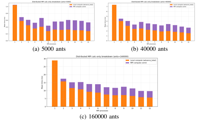
Fig. 4. MPI subdomain computation-only breakdown for selected colony sizes.
