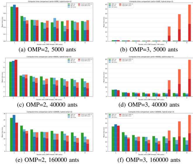
Fig. 6. Hybrid OMP-only vs MPI-only vs MPI+OpenMP computation-only comparison for selected colony sizes. The left column corresponds to two OpenMP threads per subdomain and the right column corresponds to three OpenMP threads per subdomain. The associated efficiency is computed with respect to compute MPI processes only, excluding rendering.
