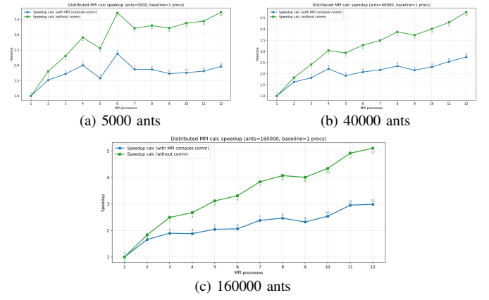
Fig. 3. MPI subdomain computation speedup (with and without communication) for selected colony sizes. The associated efficiency is computed with respect to compute MPI processes only, excluding rendering.
