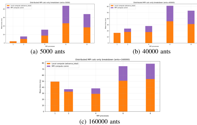
Fig. 4. MPI population computation-only breakdown for selected colony sizes.
