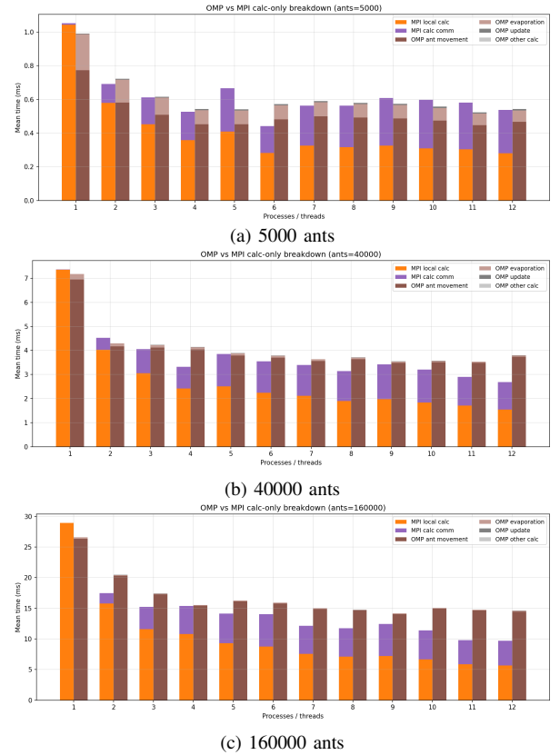
Fig. 8. MPI subdomain vs OpenMP computation-only breakdown for selected colony sizes.
