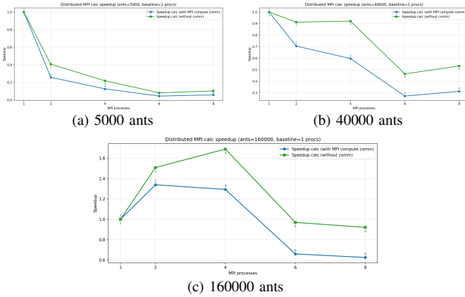
Fig. 3. MPI population computation speedup (with and without communication) for selected colony sizes.
