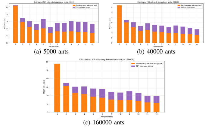
Fig. 7. MPI subdomain computation-only breakdown for selected colony sizes.
