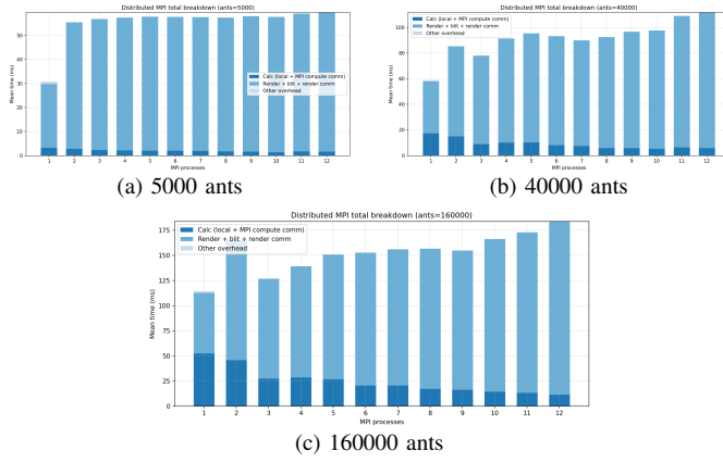
Fig. 5. MPI subdomain total iteration-time breakdown for selected colony sizes.
