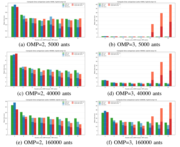
Fig. 6. Hybrid OMP-only vs MPI-only vs MPI+OpenMP computation-only comparison for selected colony sizes. The left column corresponds to two OpenMP threads per subdomain and the right column corresponds to three OpenMP threads per subdomain. The associated efficiency is computed with respect to compute MPI processes only, excluding rendering.
