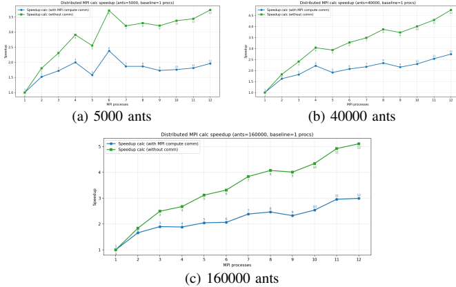
Fig. 3. MPI subdomain computation speedup (with and without communication) for selected colony sizes. The associated efficiency is computed with respect to compute MPI processes only, excluding rendering.
