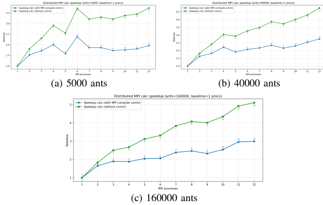
Fig. 2. MPI subdomain computation speedup (with and without communication) for selected colony sizes. The associated efficiency is computed with respect to compute MPI processes only, excluding rendering.
