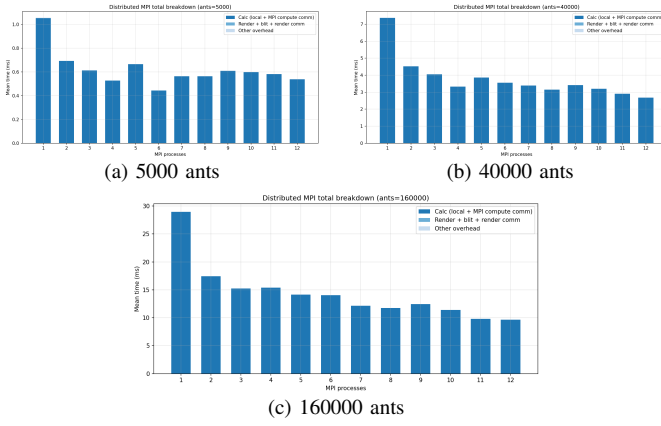
Fig. 1. MPI subdomain total iteration-time breakdown for selected colony sizes.
