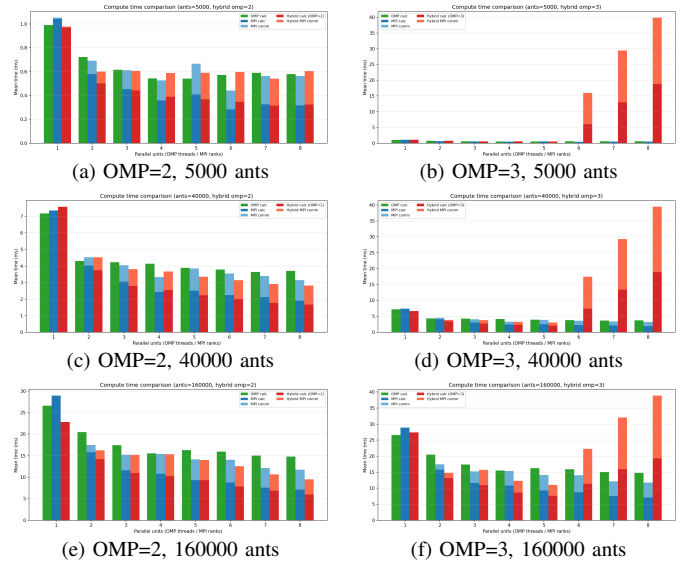
Fig. 5. Hybrid OMP-only vs MPI-only vs MPI+OpenMP computation-only comparison for selected colony sizes. The left column corresponds to two OpenMP threads per subdomain and the right column corresponds to three OpenMP threads per subdomain. The associated efficiency is computed with respect to compute MPI processes only, excluding rendering.
