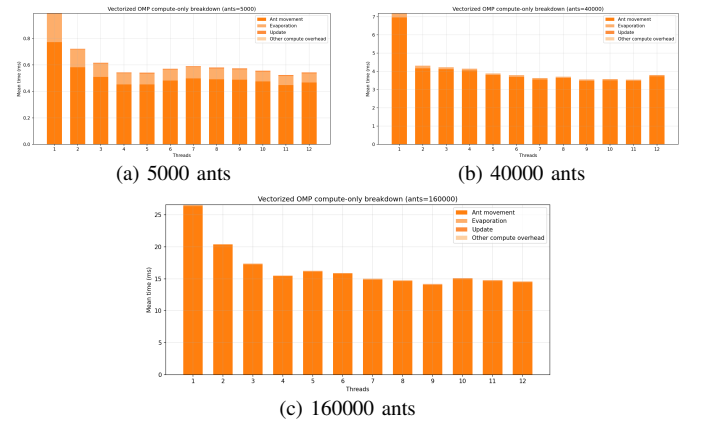
Fig. 1. Vectorized OpenMP compute-only breakdown for selected colony sizes.
