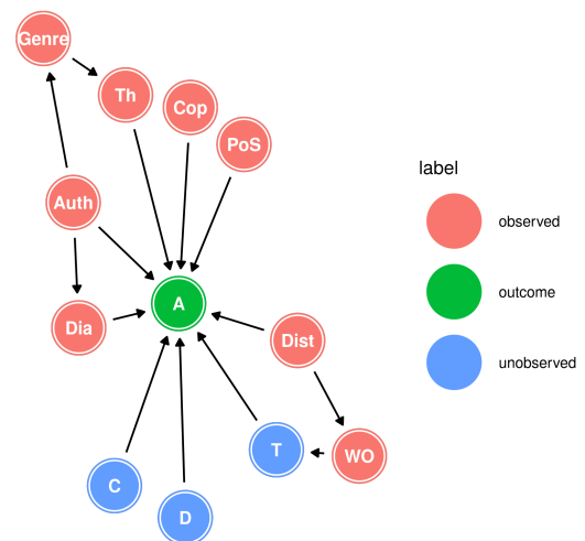
Figure 4: DAG with Attraction, Domain, Controller, Target, Part of Speech, Copula, Thematic role, Authorship, Genre, Distance, and Word Order.
