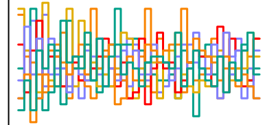
a_sent[110] n_eff = 5792
