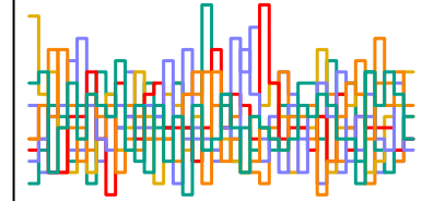
z_sent[144] n_eff = 7951
