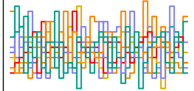
z_sent[103] n_eff = 7821
