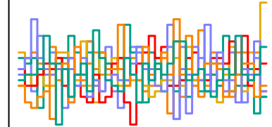
a_sent[116] n_eff = 4567
