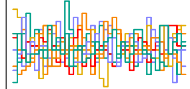
a_sent[152] n_eff = 4926
