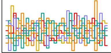
z_sent[49] n_eff = 5633
