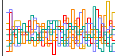
a_sent[289] n_eff = 4237
