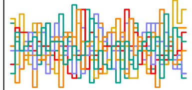
a_sent[55] n_eff = 5075
