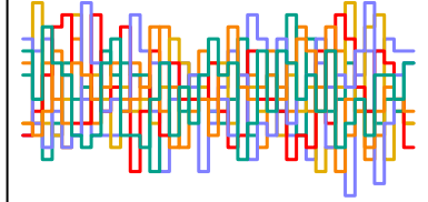
z_sent[22] n_eff = 5863
