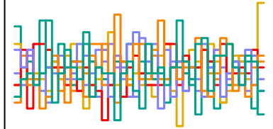
a_sent[258] n_eff = 4772
