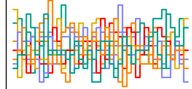
z_sent[30] n_eff = 5871
