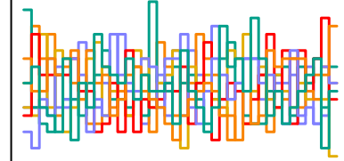
z_sent[153] n_eff = 6917
