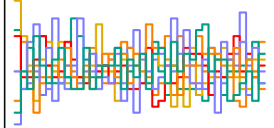
a_sent[168] n_eff = 1868
