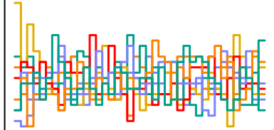
a_sent[228] n_eff = 1312
