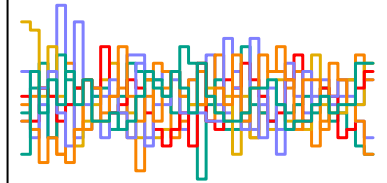
a_sent[256] n_eff = 4519
