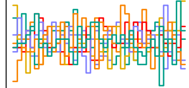
a_sent[272] n_eff = 4727
