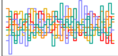
z_sent[211] n_eff = 4239
