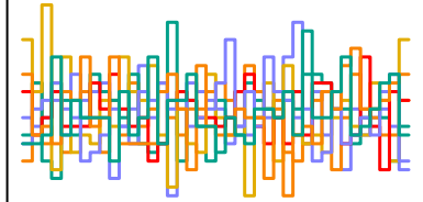
z_sent[142] n_eff = 7218
