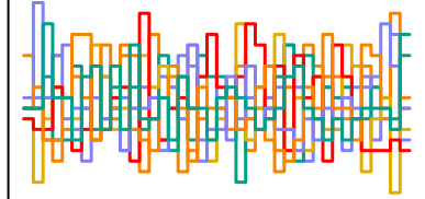
z_sent[68] n_eff = 6027
