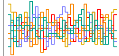
a_sent[179] n_eff = 4892
