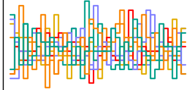
a_sent[165] n_eff = 4114
