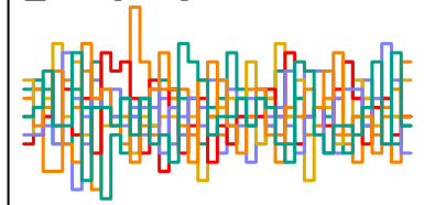
z_sent[158] n_eff = 7084
