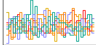
a_sent[101] n_eff = 5605
