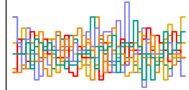
a_sent[194] n_eff = 4593
