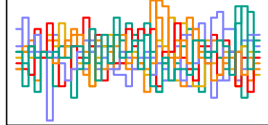
z_sent[110] n_eff = 7758
