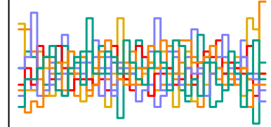
a_sent[167] n_eff = 4975
