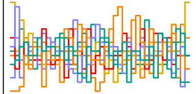
a_sent[132] n_eff = 5091
