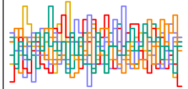
z_sent[64] n_eff = 7046
