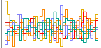
a_sent[111] n_eff = 4547
