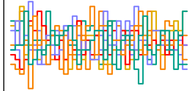
a_sent[286] n_eff = 5034
