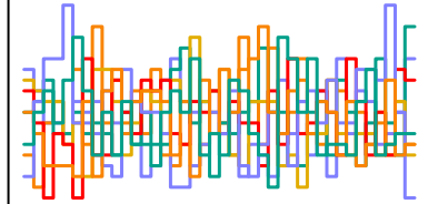
z_sent[170] n_eff = 6429
