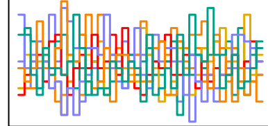
z_sent[273] n_eff = 6546
