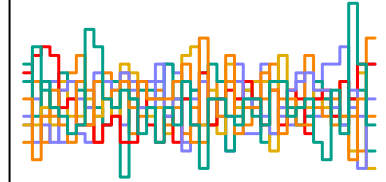
z_sent[86] n_eff = 6885
