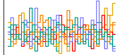
a_sent[137] n_eff = 1736
