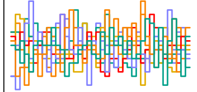
a_sent[61] n_eff = 2636
