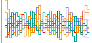
a_sent[97] n_eff = 4872
