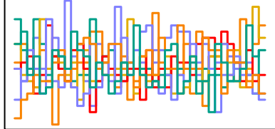
a_sent[187] n_eff = 4426
