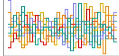
z_sent[135] n_eff = 4814
