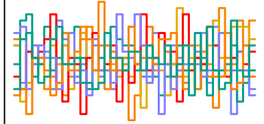
a_sent[24] n_eff = 3210
