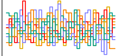
a_sent[30] n_eff = 4079
