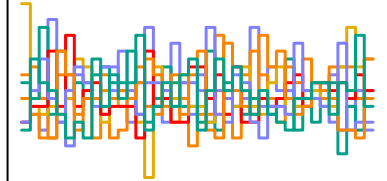
a_sent[250] n_eff = 4990
