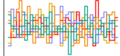
z_sent[150] n_eff = 6885
