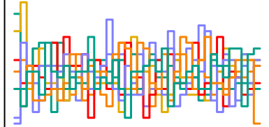
a_sent[90] n_eff = 3593
