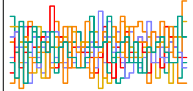
a_sent[261] n_eff = 4306
