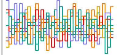
s_dia n_eff = 1956
