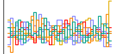
a_sent[41] n_eff = 3473
