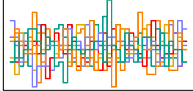
z_sent[136] n_eff = 7130
