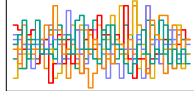
z_sent[213] n_eff = 6017
