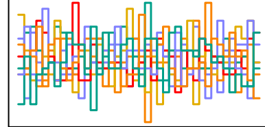
z_sent[120] n_eff = 6297
