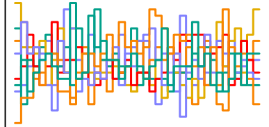
a_sent[133] n_eff = 4357
