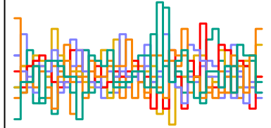
z_sent[220] n_eff = 6367
