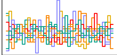
a_sent[99] n_eff = 4931
