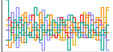
a_sent[172] n_eff = 4788
