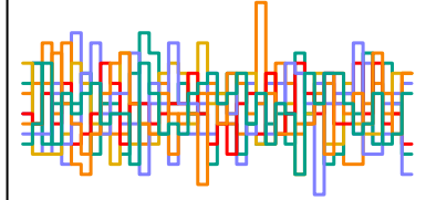
z_sent[25] n_eff = 6880
