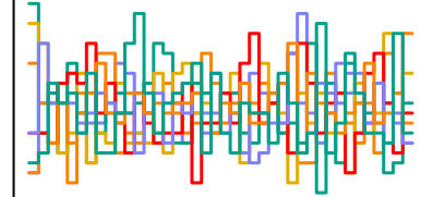
a_sent[107] n_eff = 4535
