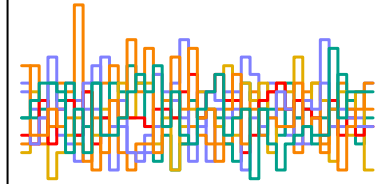
z_sent[167] n_eff = 6349
