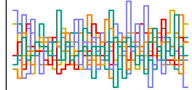
a_sent[26] n_eff = 2393
