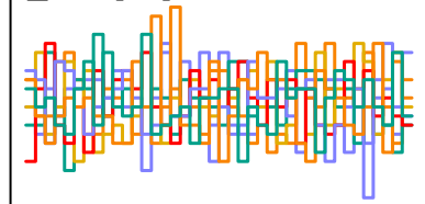
z_sent[38] n_eff = 6705
