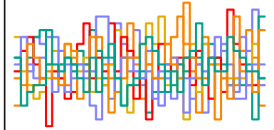
b_auth[6] n_eff = 5930
