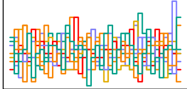
z_sent[127] n_eff = 5346
