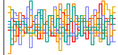
a_sent[227] n_eff = 3910
