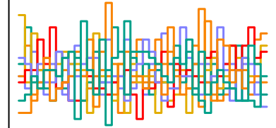
a_sent[260] n_eff = 5071
