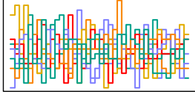
a_sent[126] n_eff = 4474
