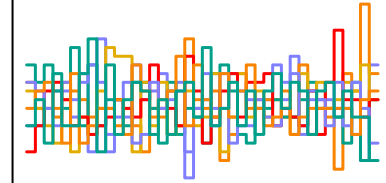
z_sent[240] n_eff = 4458
