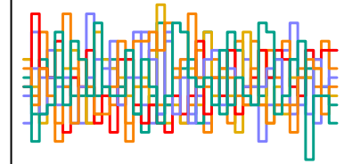
z_sent[207] n_eff = 7765
