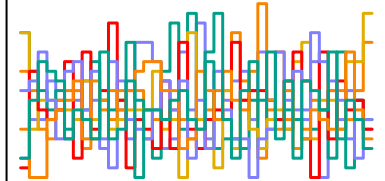
a_sent[249] n_eff = 4577
