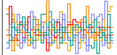
a_sent[292] n_eff = 5278
