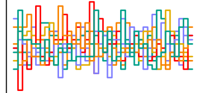
z_sent[66] n_eff = 5503
