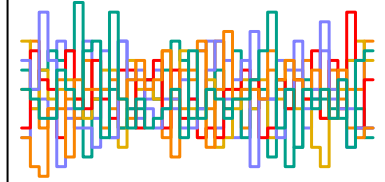
a_sent[103] n_eff = 5656
