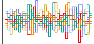
z_sent[23] n_eff = 7539
