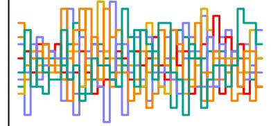
z_sent[69] n_eff = 6497
