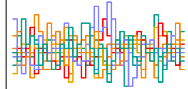
z_sent[279] n_eff = 3901
