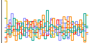
a_sent[246] n_eff = 5142
