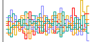
a_sent[155] n_eff = 2632
