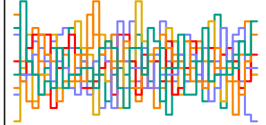
z_sent[151] n_eff = 6311
