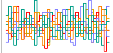
z_sent[106] n_eff = 7285
