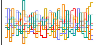
a_sent[237] n_eff = 3191
