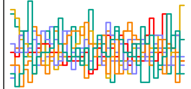
a_sent[16] n_eff = 5351
