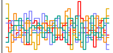
a_sent[181] n_eff = 4477
