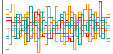
a_sent[193] n_eff = 1519
