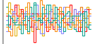
a_sent[104] n_eff = 5276
