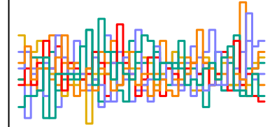
z_sent[282] n_eff = 5970
