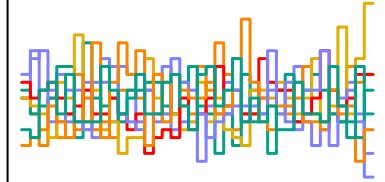
a_sent[91] n_eff = 1679
