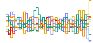
s_sent n_eff = 453
