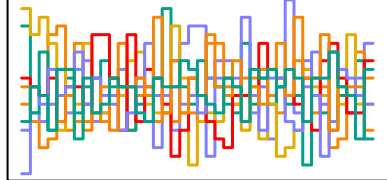
a_sent[157] n_eff = 2029
