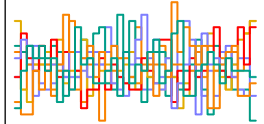
a_sent[196] n_eff = 5337
