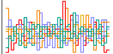
z_sent[82] n_eff = 6313
