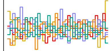
a_sent[269] n_eff = 4723
