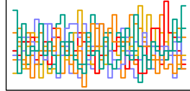
z_sent[51] n_eff = 3382
