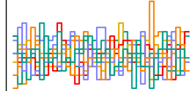
z_sent[156] n_eff = 4345
