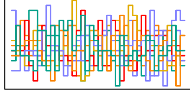
z_sent[95] n_eff = 6207
