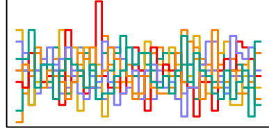
z_sent[47] n_eff = 6406
