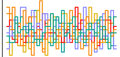
z_sent[155] n_eff = 4997
