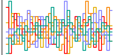
a_sent[198] n_eff = 3704
