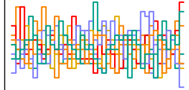
z_sent[83] n_eff = 8287
