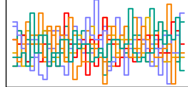
z_sent[36] n_eff = 7518
