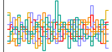
a_sent[122] n_eff = 4988
