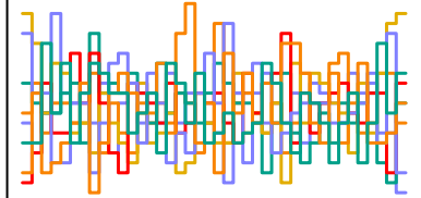
a_sent[121] n_eff = 5043
