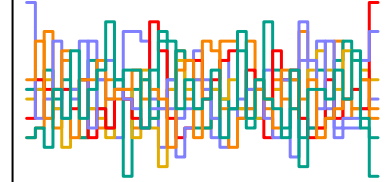
z_sent[24] n_eff = 5940
