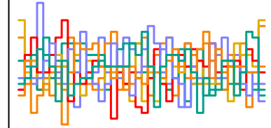
a_sent[140] n_eff = 4818
