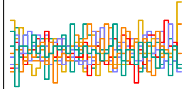
a_sent[34] n_eff = 5579
