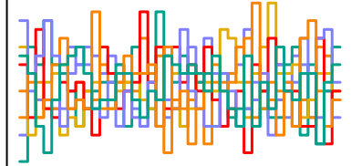
z_sent[146] n_eff = 6451
