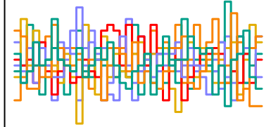
z_sent[295] n_eff = 5317
