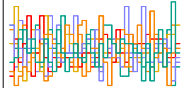
a_sent[141] n_eff = 4309
