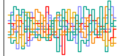
z_sent[57] n_eff = 7995
