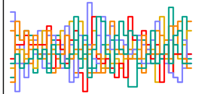
z_sent[235] n_eff = 7338
