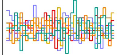
z_sent[80] n_eff = 2543
