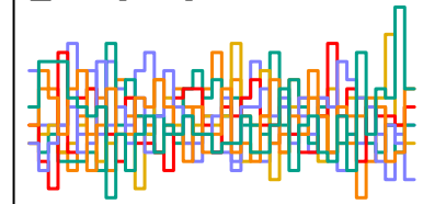
z_sent[204] n_eff = 5122
