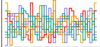
a_sent[186] n_eff = 4678
