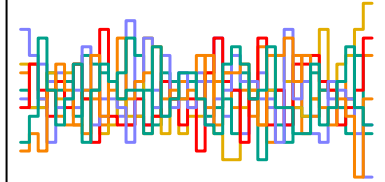
a_sent[285] n_eff = 2393
