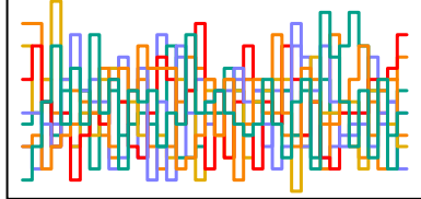
z_sent[133] n_eff = 6915
