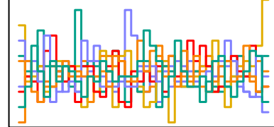
a_sent[176] n_eff = 3964
