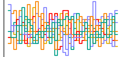
z_sent[165] n_eff = 5805
