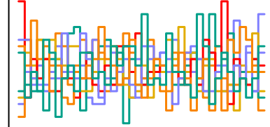
z_sent[243] n_eff = 4922
