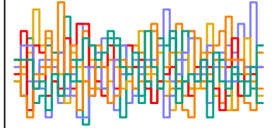
z_sent[145] n_eff = 4077
