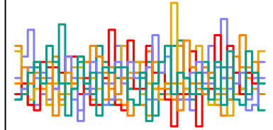
z_sent[269] n_eff = 5215
