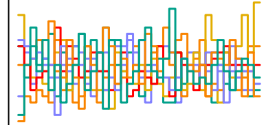
a_sent[146] n_eff = 5147
