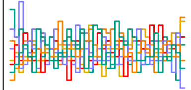
a_sent[240] n_eff = 2667
