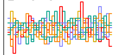
z_sent[159] n_eff = 5466
