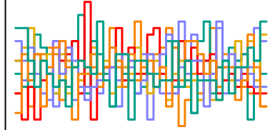
z_sent[245] n_eff = 5236
