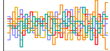
z_sent[228] n_eff = 2695
