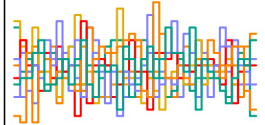
a_sent[105] n_eff = 4866
