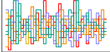
z_sent[88] n_eff = 6748
