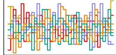
a_sent[14] n_eff = 4574
