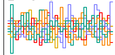
z_sent[234] n_eff = 6672
