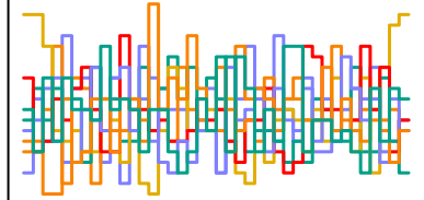
a_sent[295] n_eff = 3942
