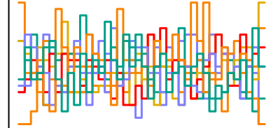
a_sent[296] n_eff = 5268
