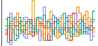
z_sent[67] n_eff = 8001
