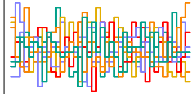
z_sent[266] n_eff = 2843
