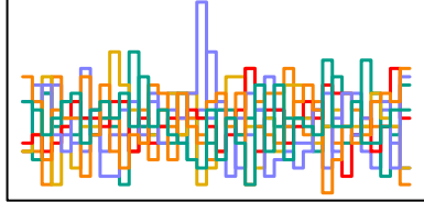
z_sent[121] n_eff = 5839
