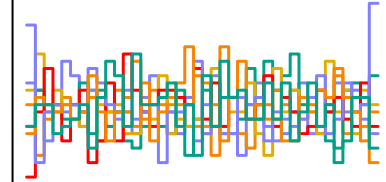
z_sent[87] n_eff = 6538
