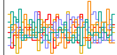
z_sent[219] n_eff = 7010
