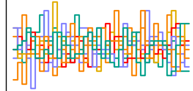
a_sent[200] n_eff = 4951
