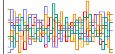
a_sent[233] n_eff = 2172
