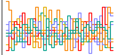
z_sent[166] n_eff = 7556
