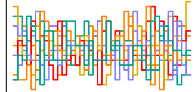
a_sent[32] n_eff = 5110
