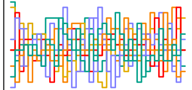
a_sent[229] n_eff = 5025
