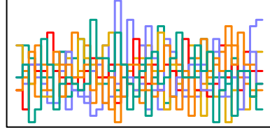
z_sent[92] n_eff = 5988
