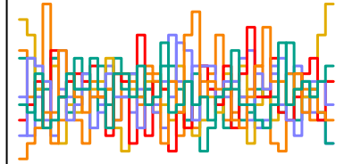
a_sent[88] n_eff = 4552
