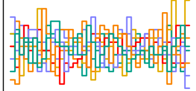
a_sent[279] n_eff = 2403
