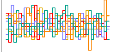
z_sent[31] n_eff = 6818
