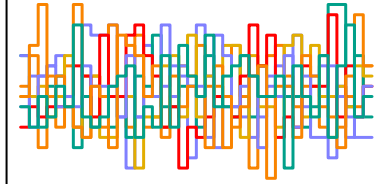
z_sent[52] n_eff = 5479
