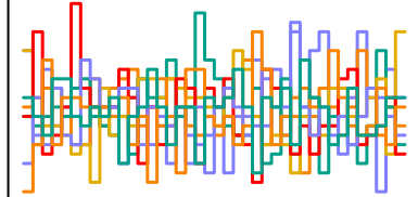
z_sent[221] n_eff = 5882
