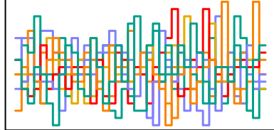
z_sent[128] n_eff = 5266
