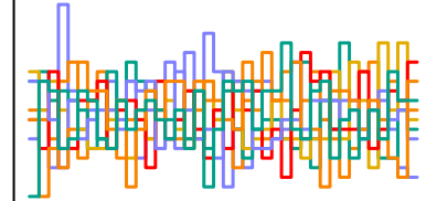
a_sent[185] n_eff = 5481
