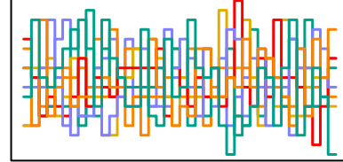
z_sent[96] n_eff = 7267
