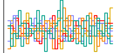
a_sent[278] n_eff = 4899
