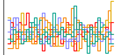
a_sent[89] n_eff = 3750
