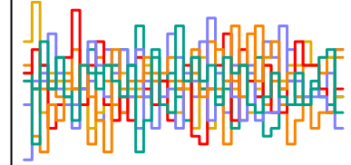
a_sent[239] n_eff = 5092
