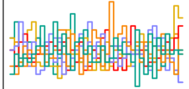
a_sent[204] n_eff = 3496
