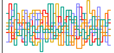
z_sent[131] n_eff = 6617
