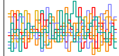
z_sent[270] n_eff = 3593
