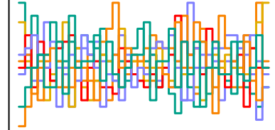
a_sent[143] n_eff = 4976
