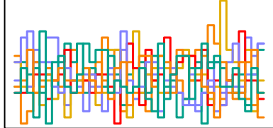
z_sent[226] n_eff = 5986
