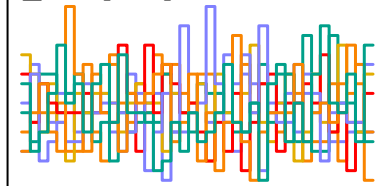
z_sent[113] n_eff = 5737
