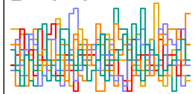
z_sent[263] n_eff = 3257
