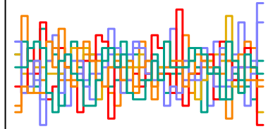
z_sent[53] n_eff = 5033
