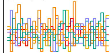
z_sent[39] n_eff = 6589
