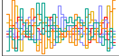
z_sent[134] n_eff = 7034
