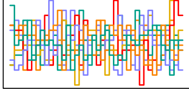
z_sent[91] n_eff = 3463
