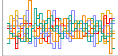
z_sent[89] n_eff = 5626
