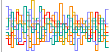
z_sent[28] n_eff = 7273
