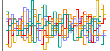
a_sent[70] n_eff = 1964
