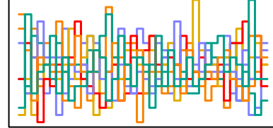
z_sent[138] n_eff = 5045
