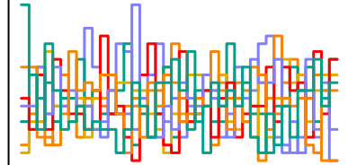
z_sent[41] n_eff = 5477
