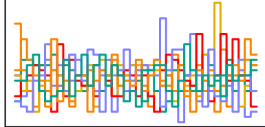
z_sent[119] n_eff = 6749
