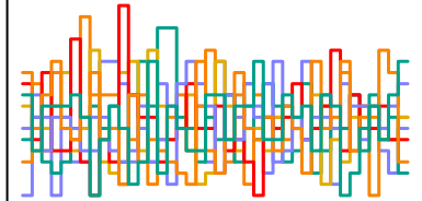
z_sent[163] n_eff = 7310
