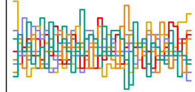
a_sent[164] n_eff = 2699
