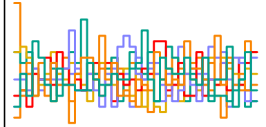
a_sent[222] n_eff = 5224
