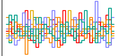
z_sent[277] n_eff = 5943
