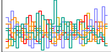
z_sent[289] n_eff = 6327
