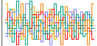
z_sent[209] n_eff = 5546
