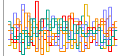
z_sent[63] n_eff = 7034
