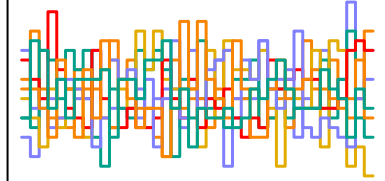
z_sent[224] n_eff = 6517
