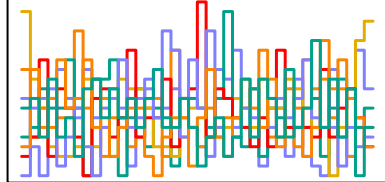
z_sent[212] n_eff = 6475
