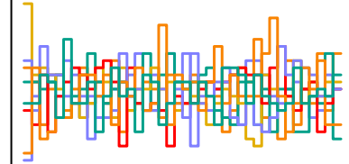
a_sent[245] n_eff = 3280
