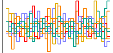
z_sent[281] n_eff = 5907
