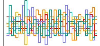
z_sent[72] n_eff = 7475
