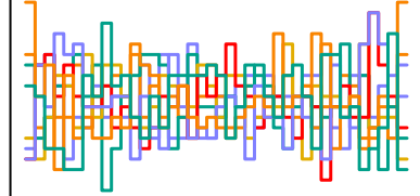
z_sent[104] n_eff = 6453
