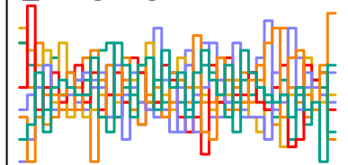
a_sent[253] n_eff = 2001
