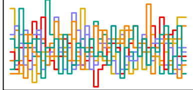
a_sent[175] n_eff = 5507
