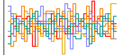
a_sent[251] n_eff = 4800
