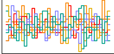
a_sent[127] n_eff = 3772
