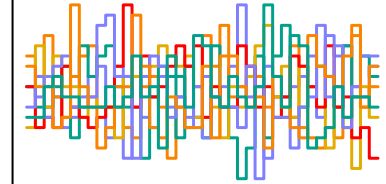
z_sent[168] n_eff = 3611
