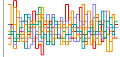
z_sent[216] n_eff = 5998
