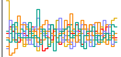
a_sent[102] n_eff = 5573
