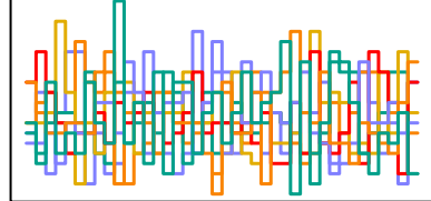
z_sent[107] n_eff = 6403
