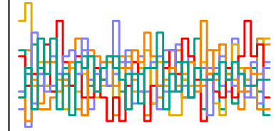
a_sent[224] n_eff = 3804
