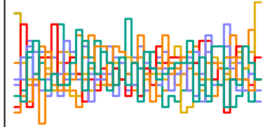
a_sent[195] n_eff = 4778
