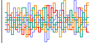
z_sent[71] n_eff = 6561
