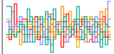
z_sent[143] n_eff = 5827
