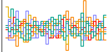
a_sent[163] n_eff = 3693
