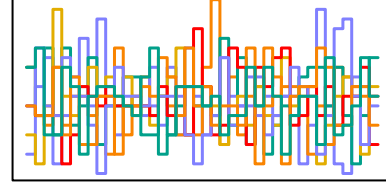
z_sent[141] n_eff = 6788
