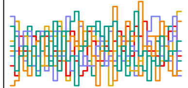
a_sent[136] n_eff = 4748
