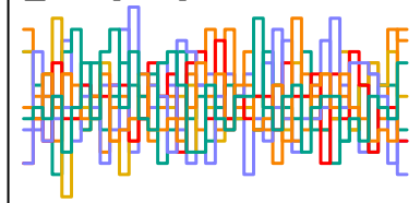
z_sent[203] n_eff = 6496
