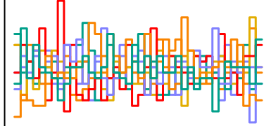
a_sent[48] n_eff = 5549
