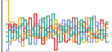
a_sent[174] n_eff = 2219
