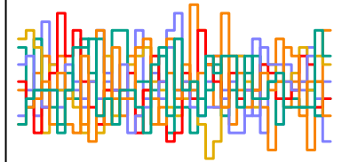
a_sent[255] n_eff = 5184
