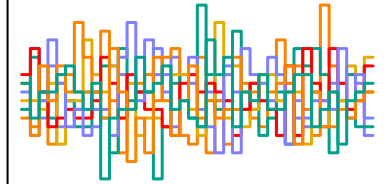
z_sent[164] n_eff = 4513
