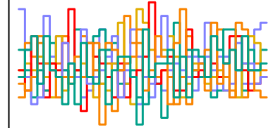
z_sent[102] n_eff = 7347
