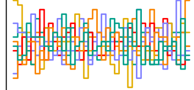
a_sent[68] n_eff = 5176
