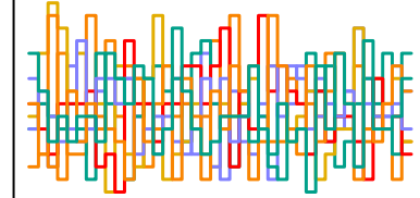
z_sent[246] n_eff = 7581
