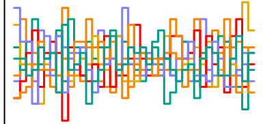
a_sent[135] n_eff = 3777
