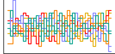
a_sent[128] n_eff = 2616
