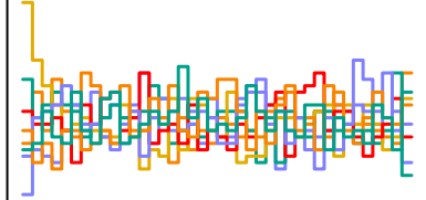
a_sent[270] n_eff = 1862
