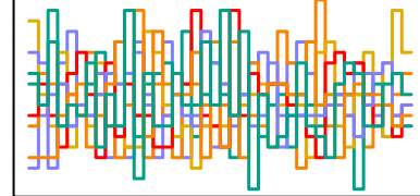
a_sent[173] n_eff = 4940
