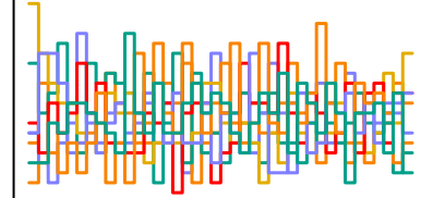
a_sent[92] n_eff = 3811
