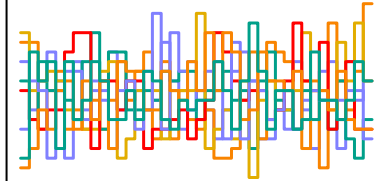
a_sent[114] n_eff = 4764
