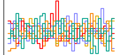
a_sent[287] n_eff = 4398
