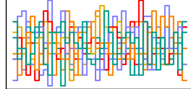
z_sent[111] n_eff = 6969
