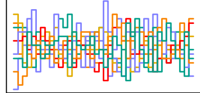
a_sent[125] n_eff = 5615
