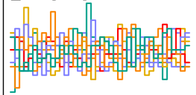
z_sent[262] n_eff = 6737
