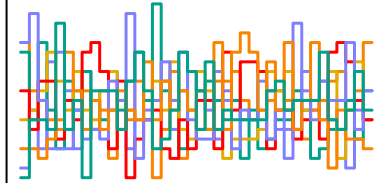
a_sent[36] n_eff = 5235
