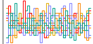
a_sent[230] n_eff = 4530
