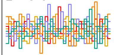
z_sent[37] n_eff = 6596
