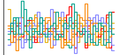
a_sent[35] n_eff = 5195
