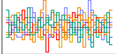
a_sent[96] n_eff = 5081
