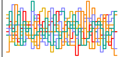
z_sent[268] n_eff = 6611
