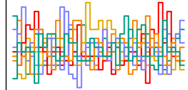
z_sent[117] n_eff = 6661
