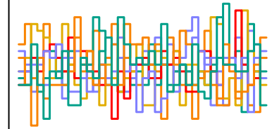
z_sent[162] n_eff = 5500
