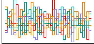
z_sent[140] n_eff = 5732
