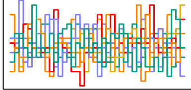
a_sent[129] n_eff = 1686
