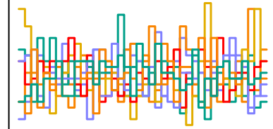
a_sent[134] n_eff = 4961
