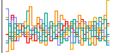
a_sent[273] n_eff = 3684
