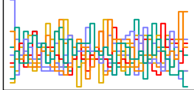
z_sent[34] n_eff = 7021
