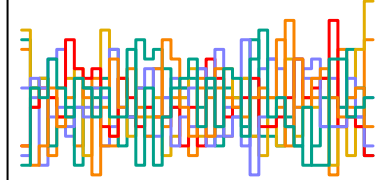
a_sent[64] n_eff = 5014
