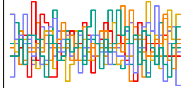
a_sent[205] n_eff = 5388
