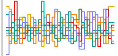
a_sent[291] n_eff = 4953
