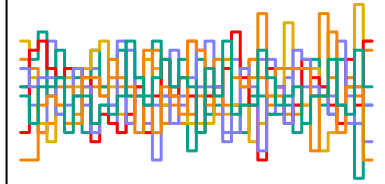
a_sent[117] n_eff = 5438
