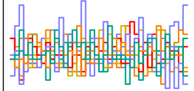
z_sent[241] n_eff = 6529
