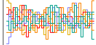
a_sent[197] n_eff = 2944
