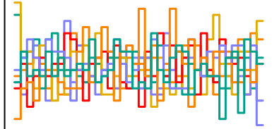
a_sent[144] n_eff = 5026
