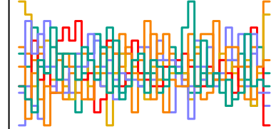
a_sent[20] n_eff = 4957
