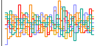
a_sent[294] n_eff = 5478
