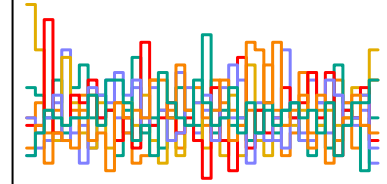
a_sent[284] n_eff = 5268
