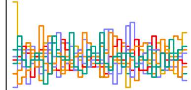
a_sent[293] n_eff = 4783
