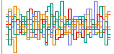
a_sent[108] n_eff = 5277
