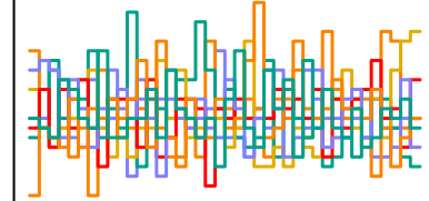
a_sent[47] n_eff = 3698
