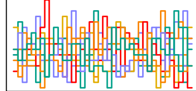
z_sent[33] n_eff = 6096
