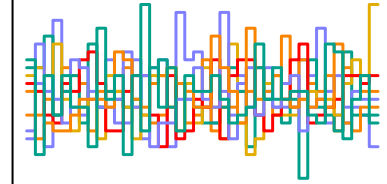
a_sent[29] n_eff = 4805
