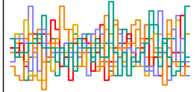
z_sent[55] n_eff = 6403
