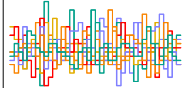
z_sent[100] n_eff = 8677
