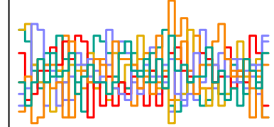
a_sent[53] n_eff = 2892
