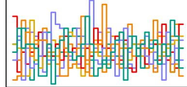
z_sent[288] n_eff = 6435
