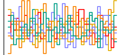
z_sent[27] n_eff = 6935
