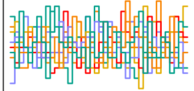
a_sent[15] n_eff = 4991
