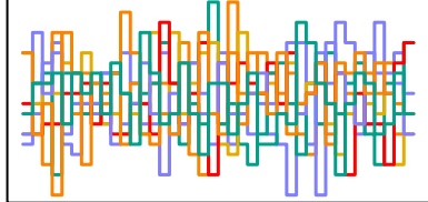
z_sent[271] n_eff = 3640
