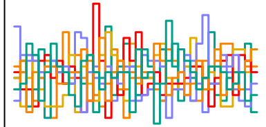
z_sent[115] n_eff = 5276
