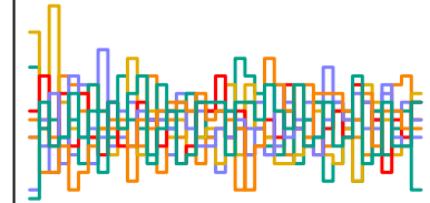
a_sent[182] n_eff = 2595
