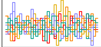
z_sent[227] n_eff = 5763
