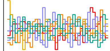
a_sent[95] n_eff = 4658
