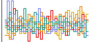
a_sent[115] n_eff = 3369
