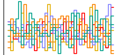
z_sent[237] n_eff = 5049
