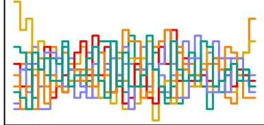
a_sent[12] n_eff = 2041
