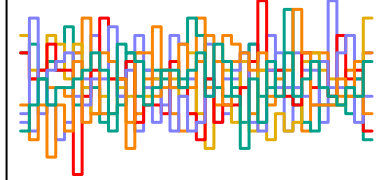
a_sent[54] n_eff = 2633
