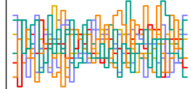
z_sent[132] n_eff = 5773
