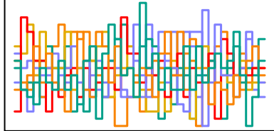
z_sent[43] n_eff = 6015
