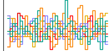
a_sent[50] n_eff = 4501
