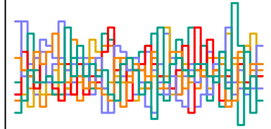
z_sent[218] n_eff = 6111
