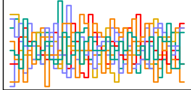
a_sent[124] n_eff = 4430
