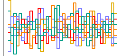
a_sent[98] n_eff = 4952
