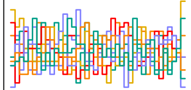
a_sent[268] n_eff = 3601
