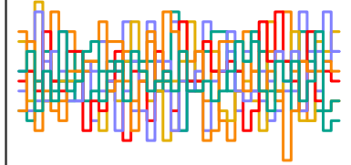
z_sent[148] n_eff = 6593
