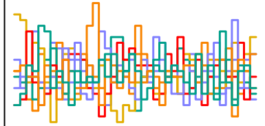
z_sent[97] n_eff = 7384
