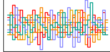
z_sent[93] n_eff = 7169
