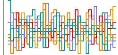
a_sent[170] n_eff = 5180
