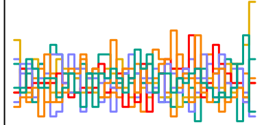
a_sent[264] n_eff = 3687
