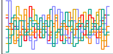
z_sent[274] n_eff = 6291
