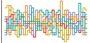
a_sent[87] n_eff = 5343
