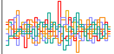
z_sent[217] n_eff = 7605
