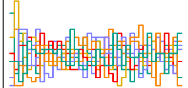
a_sent[60] n_eff = 2277
