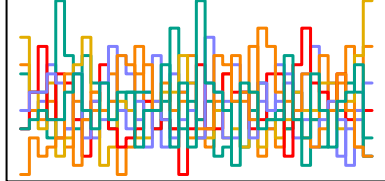
a_sent[189] n_eff = 5376
