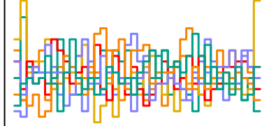
a_sent[66] n_eff = 3018
