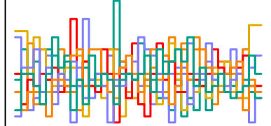
a_sent[154] n_eff = 5181
