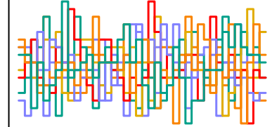
z_sent[105] n_eff = 7040
