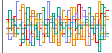
z_sent[161] n_eff = 7391
