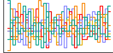
z_sent[48] n_eff = 6772
