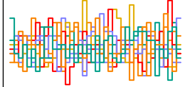
z_sent[73] n_eff = 5441
