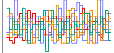
z_sent[32] n_eff = 5881
