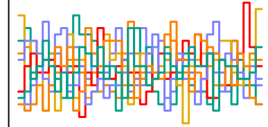
a_sent[38] n_eff = 5299
