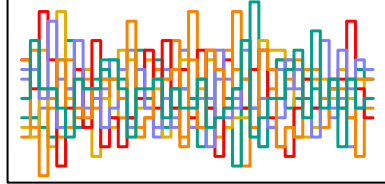
z_sent[122] n_eff = 7118
