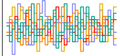
z_sent[284] n_eff = 7716
