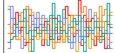
a_sent[65] n_eff = 5233
