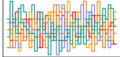
z_sent[44] n_eff = 7080
