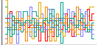
a_sent[100] n_eff = 5391
