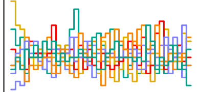
a_sent[271] n_eff = 1832
