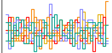
z_sent[265] n_eff = 5392
