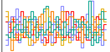
a_sent[288] n_eff = 4376
