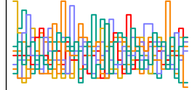
a_sent[149] n_eff = 4488
