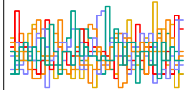
z_sent[239] n_eff = 6795
