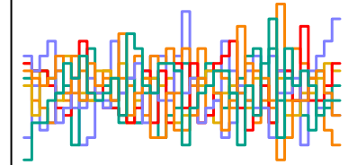
z_sent[99] n_eff = 7822
