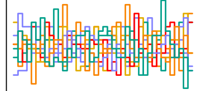
z_sent[81] n_eff = 7338
