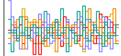
z_sent[285] n_eff = 3798
