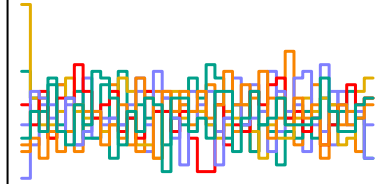
a_sent[283] n_eff = 4336
