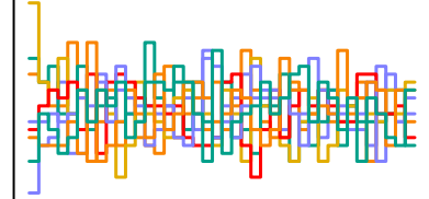
a_sent[266] n_eff = 1775
