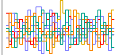
z_sent[130] n_eff = 3853
