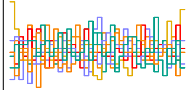
a_sent[234] n_eff = 5250
