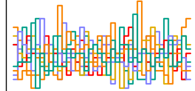
a_sent[59] n_eff = 4584
