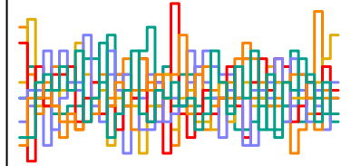
a_sent[37] n_eff = 4936
