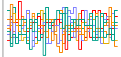
z_sent[98] n_eff = 6200
