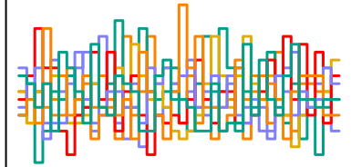
z_sent[40] n_eff = 5830
