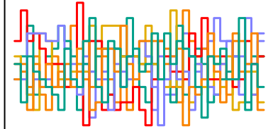
z_sent[61] n_eff = 4572
