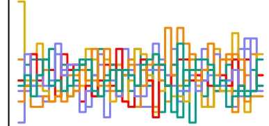
a_sent[62] n_eff = 2540
