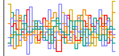
a_sent[119] n_eff = 5267
