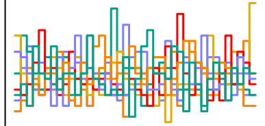
a_sent[28] n_eff = 5015
