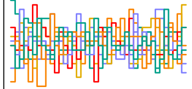
a_sent[280] n_eff = 5095
