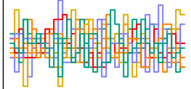
z_sent[79] n_eff = 6071
