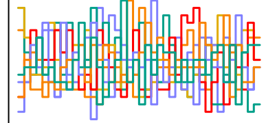
a_sent[71] n_eff = 5220
