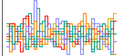
a_sent[46] n_eff = 5390
