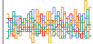
a_sent[44] n_eff = 5827
