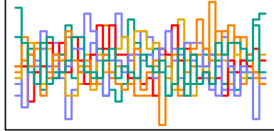
z_sent[125] n_eff = 7405
