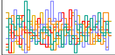
z_sent[118] n_eff = 6485
