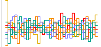
a_sent[13] n_eff = 4043
