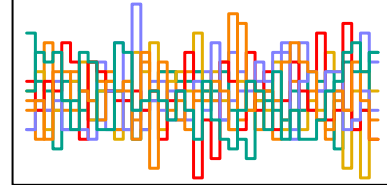
z_sent[45] n_eff = 3250
