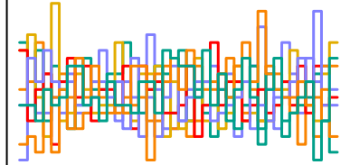
a_sent[145] n_eff = 2844
