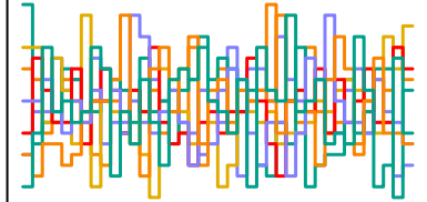
a_sent[183] n_eff = 5112
