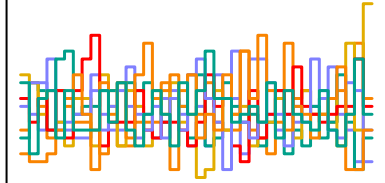
a_sent[39] n_eff = 5408
