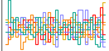
a_sent[276] n_eff = 2739
