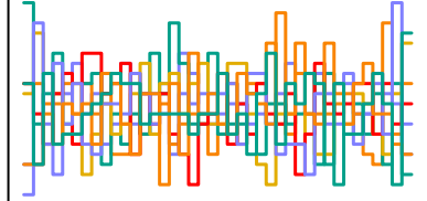
a_sent[238] n_eff = 2960
