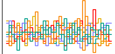
z_sent[149] n_eff = 5863
