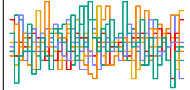
z_sent[85] n_eff = 7709
