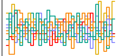
a_sent[118] n_eff = 4535
