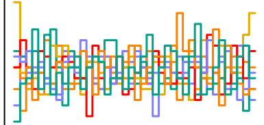
a_sent[120] n_eff = 4862
