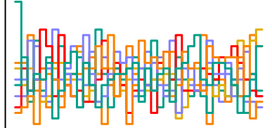
a_sent[58] n_eff = 4232
