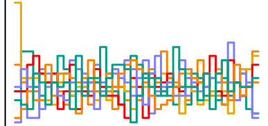
a_sent[142] n_eff = 5320
