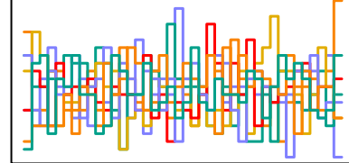
a_sent[191] n_eff = 4822
