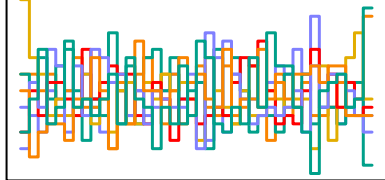
a_sent[159] n_eff = 3092
