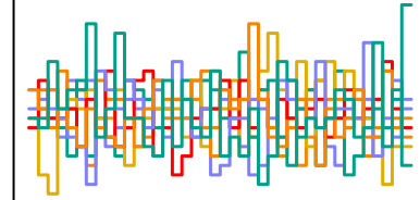
z_sent[84] n_eff = 7557
