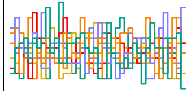
z_sent[206] n_eff = 6810
