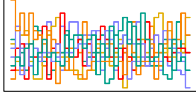
z_sent[137] n_eff = 2963
