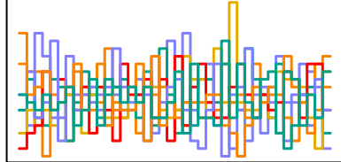
z_sent[215] n_eff = 5492
