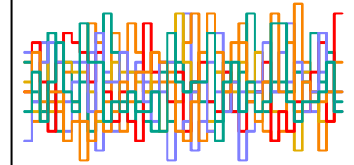
z_sent[60] n_eff = 4484
