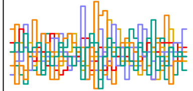
z_sent[280] n_eff = 6797
