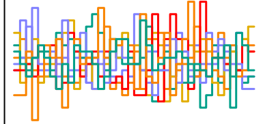
a_sent[147] n_eff = 5390
