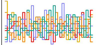
a_sent[178] n_eff = 5229
