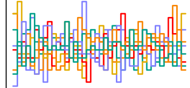
a_sent[242] n_eff = 3887
