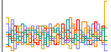
a_sent[259] n_eff = 4005
