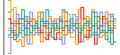
a_sent[263] n_eff = 1860
