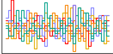
z_sent[94] n_eff = 7580
