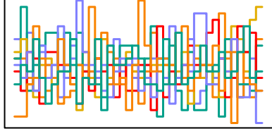
a_sent[130] n_eff = 2509
