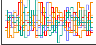
z_sent[139] n_eff = 7248
