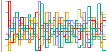
z_sent[58] n_eff = 5811
