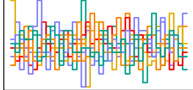
z_sent[287] n_eff = 5940
