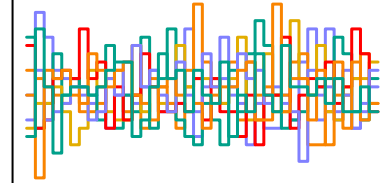
z_sent[210] n_eff = 5813
