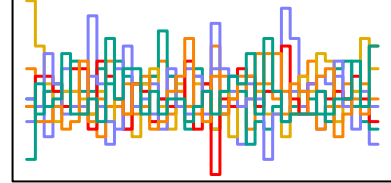
a_sent[131] n_eff = 4764
