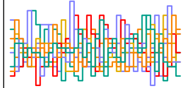
d_noun n_eff = 4712
