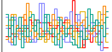
z_sent[223] n_eff = 4964
