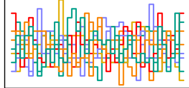
z_sent[35] n_eff = 6532
