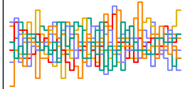
a_sent[27] n_eff = 5337
