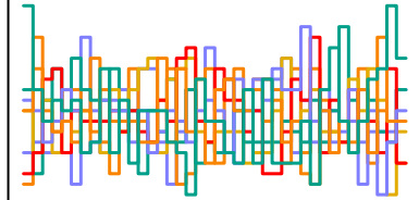
z_sent[236] n_eff = 6706
