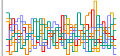
a_sent[225] n_eff = 4982
