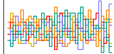
z_sent[222] n_eff = 6177
