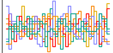
a_sent[112] n_eff = 5079
