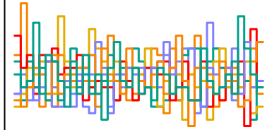
z_sent[169] n_eff = 2610
