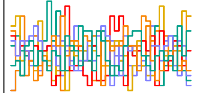
a_sent[151] n_eff = 5061
