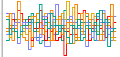
z_sent[208] n_eff = 4925
