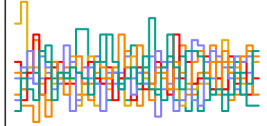
a_sent[43] n_eff = 3529
