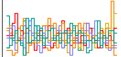
a_sent[235] n_eff = 4635
