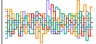
z_sent[74] n_eff = 7817
