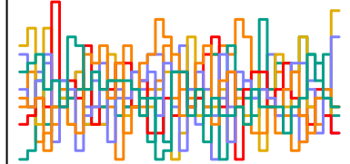
z_dia[1] n_eff = 3331
