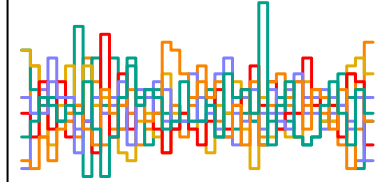
a_sent[25] n_eff = 5031
