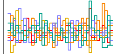
z_sent[147] n_eff = 7172
