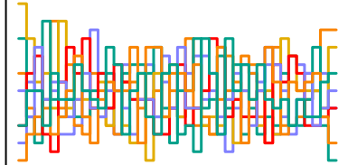
a_sent[33] n_eff = 4088
