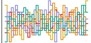
a_sent[31] n_eff = 5149
