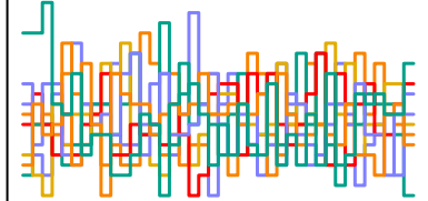
z_sent[70] n_eff = 4209
