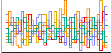
z_sent[46] n_eff = 6456
