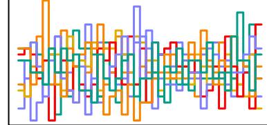
z_sent[291] n_eff = 6918
