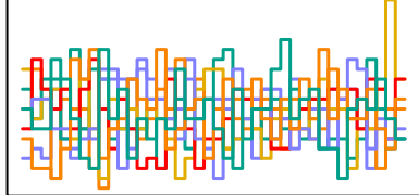
a_sent[171] n_eff = 4931
