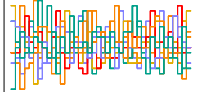
a_sent[67] n_eff = 5523
