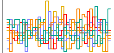
z_sent[101] n_eff = 8200
