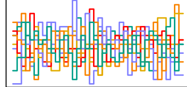
z_sent[231] n_eff = 3776
