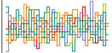
a_sent[192] n_eff = 5133
