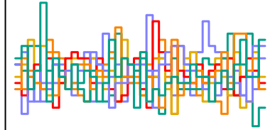
z_sent[62] n_eff = 5199
