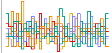
z_sent[238] n_eff = 5380
