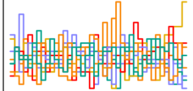
a_sent[231] n_eff = 2044
