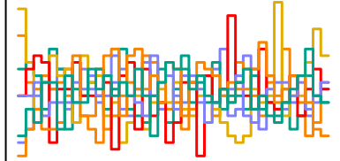
a_sent[162] n_eff = 4565
