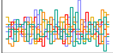
a_sent[190] n_eff = 4422
