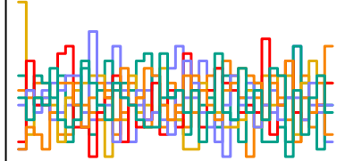
a_sent[166] n_eff = 5771
