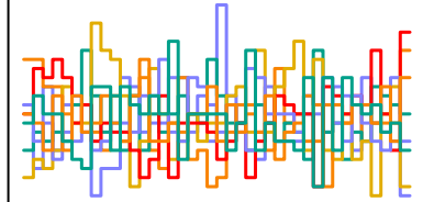
z_sent[278] n_eff = 7270
