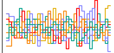
a_sent[274] n_eff = 4763
