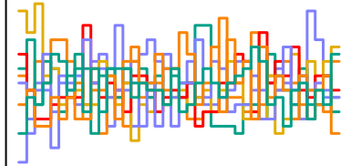
a_sent[243] n_eff = 2937
