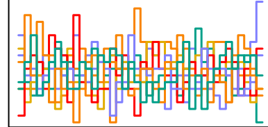
z_sent[129] n_eff = 3159
