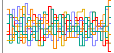
z_sent[26] n_eff = 4960
