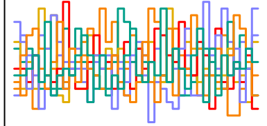
z_sent[154] n_eff = 6547
