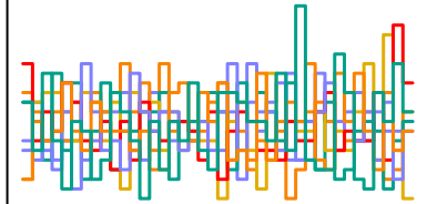
z_sent[160] n_eff = 6572
