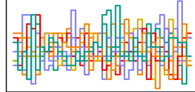
z_sent[90] n_eff = 5872
