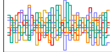
z_sent[108] n_eff = 6651
