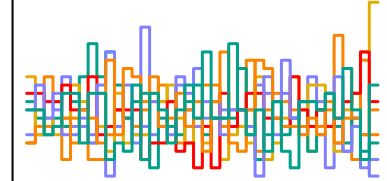
a_sent[17] n_eff = 3411
