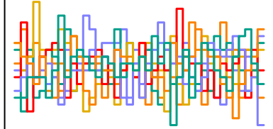
z_sent[244] n_eff = 5072
