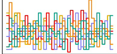
a_sent[160] n_eff = 3433
