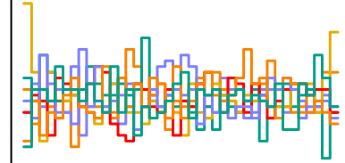
a_sent[203] n_eff = 4865
