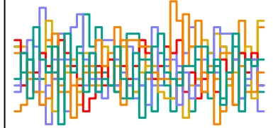
a_sent[21] n_eff = 5729
