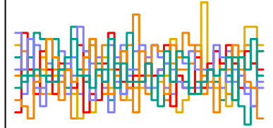
a_sent[226] n_eff = 4234
