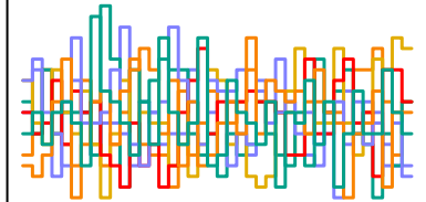
a_sent[180] n_eff = 1418
