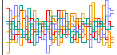
z_sent[230] n_eff = 5432
