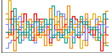
a_sent[123] n_eff = 2963
