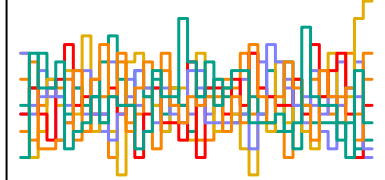
a_sent[63] n_eff = 3733
