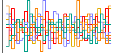
a_sent[19] n_eff = 5064
