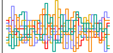
z_sent[152] n_eff = 6869
