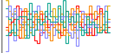
a_sent[150] n_eff = 4256
