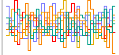
z_sent[76] n_eff = 5728
