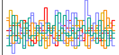
z_sent[77] n_eff = 6121
