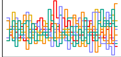
z_sent[275] n_eff = 5774
