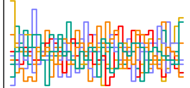
a_sent[22] n_eff = 3468
