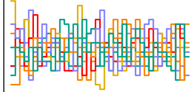
a_sent[262] n_eff = 4023
