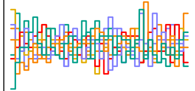
a_sent[244] n_eff = 3173
