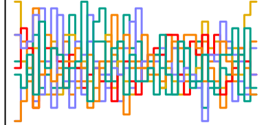
a_sent[148] n_eff = 5236
