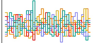
a_sent[106] n_eff = 5266
