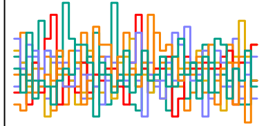
a_sent[138] n_eff = 3280
