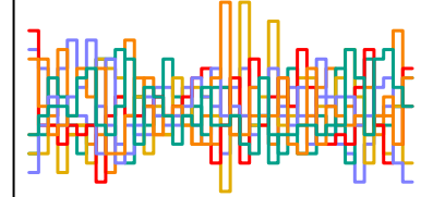
z_sent[225] n_eff = 6858
