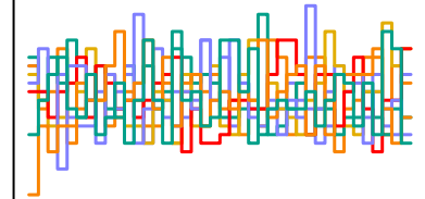
a_sent[257] n_eff = 4196
