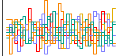
z_sent[272] n_eff = 6548
