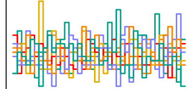
z_sent[294] n_eff = 6530
