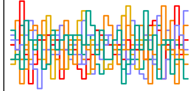
z_sent[296] n_eff = 6806
