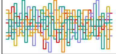
z_sent[286] n_eff = 7266
