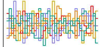
z_sent[54] n_eff = 3819
