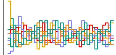
a_sent[236] n_eff = 4116
