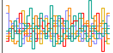
z_sent[242] n_eff = 6139
