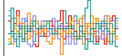
z_sent[75] n_eff = 7714
