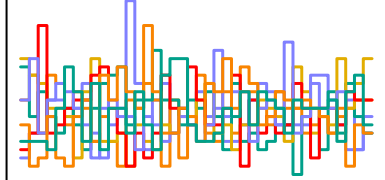
a_sent[69] n_eff = 5085
