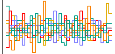
a_sent[199] n_eff = 5333
