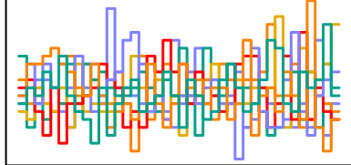
z_sent[109] n_eff = 2533
