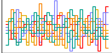
z_sent[214] n_eff = 8172
