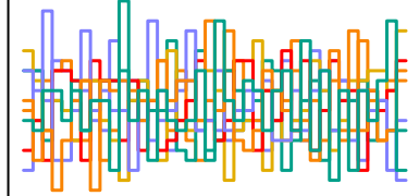
a_sent[52] n_eff = 4491
