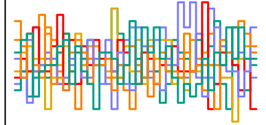
z_sent[56] n_eff = 3668
