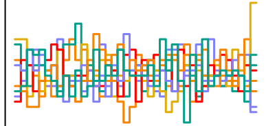
a_sent[139] n_eff = 4921
