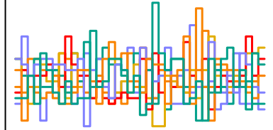
a_sent[202] n_eff = 4725
