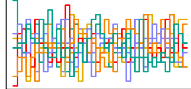
a_sent[188] n_eff = 4902
