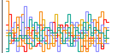
z_sent[59] n_eff = 6556
