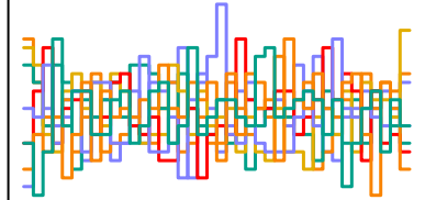
a_sent[247] n_eff = 4968
