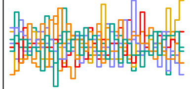
a_sent[51] n_eff = 1881
