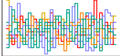
z_sent[229] n_eff = 5760
