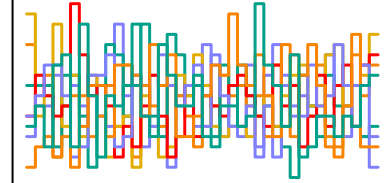
a_sent[206] n_eff = 5011
