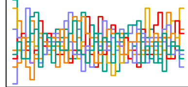
a_sent[161] n_eff = 5139
