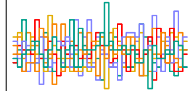
z_sent[267] n_eff = 6055
