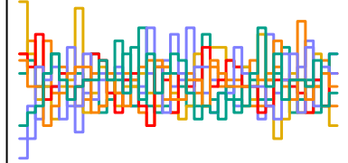
b_dist n_eff = 1234
