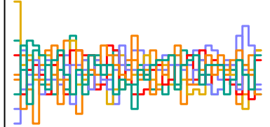
a_sent[45] n_eff = 1625
