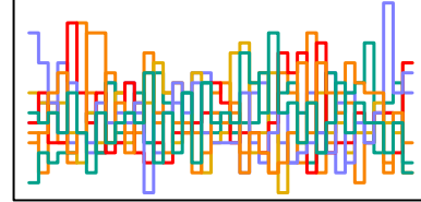
z_sent[126] n_eff = 7370
