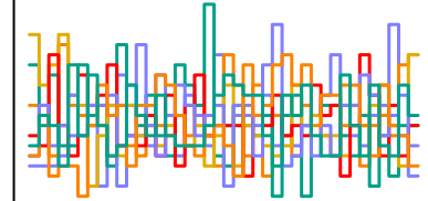
a_sent[248] n_eff = 3296
