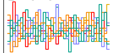
a_sent[254] n_eff = 5466
