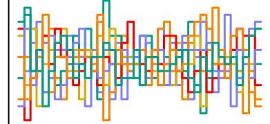
z_sent[78] n_eff = 7105
