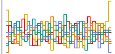
a_sent[201] n_eff = 5083
