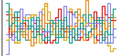
z_sent[283] n_eff = 6234
