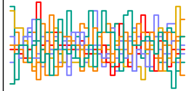
a_sent[282] n_eff = 5141
