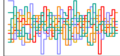
z_sent[276] n_eff = 4254
