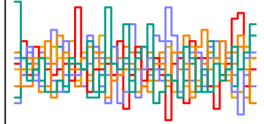
z_sent[293] n_eff = 6717
