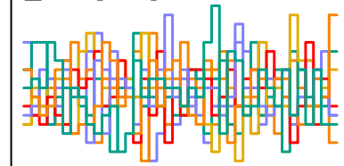
z_sent[264] n_eff = 5378
