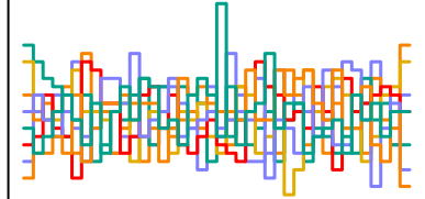
a_sent[241] n_eff = 4165
