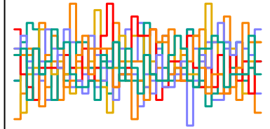
z_sent[205] n_eff = 7182
