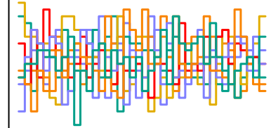
a_sent[113] n_eff = 3513
