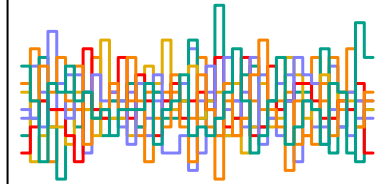
z_sent[116] n_eff = 6242
