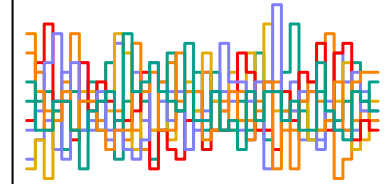
z_sent[171] n_eff = 6801
