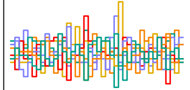
z_sent[65] n_eff = 7471
