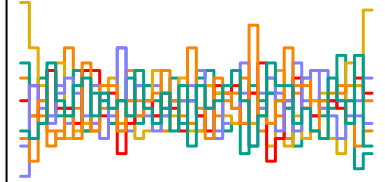
a_sent[267] n_eff = 4406
