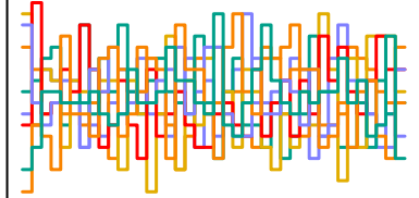
a_sent[42] n_eff = 4860
