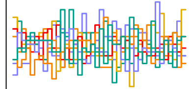
a_sent[290] n_eff = 4203
