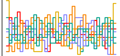
a_sent[93] n_eff = 5463
