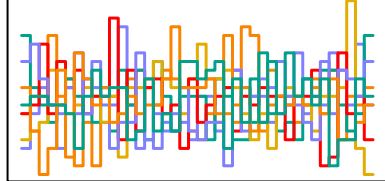
z_sent[290] n_eff = 6909
