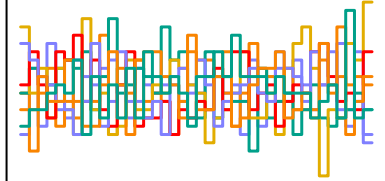
a_sent[18] n_eff = 5216
