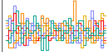
a_sent[40] n_eff = 4746
