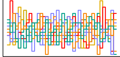
z_sent[50] n_eff = 5703
