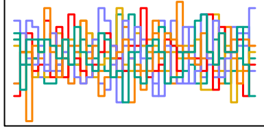
z_sent[124] n_eff = 6045
