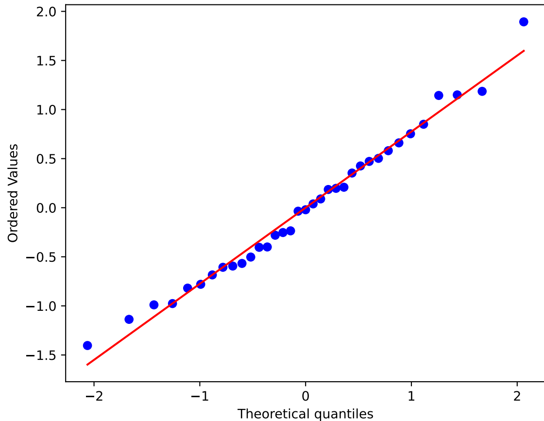
Q-Q Plot of Residuals
