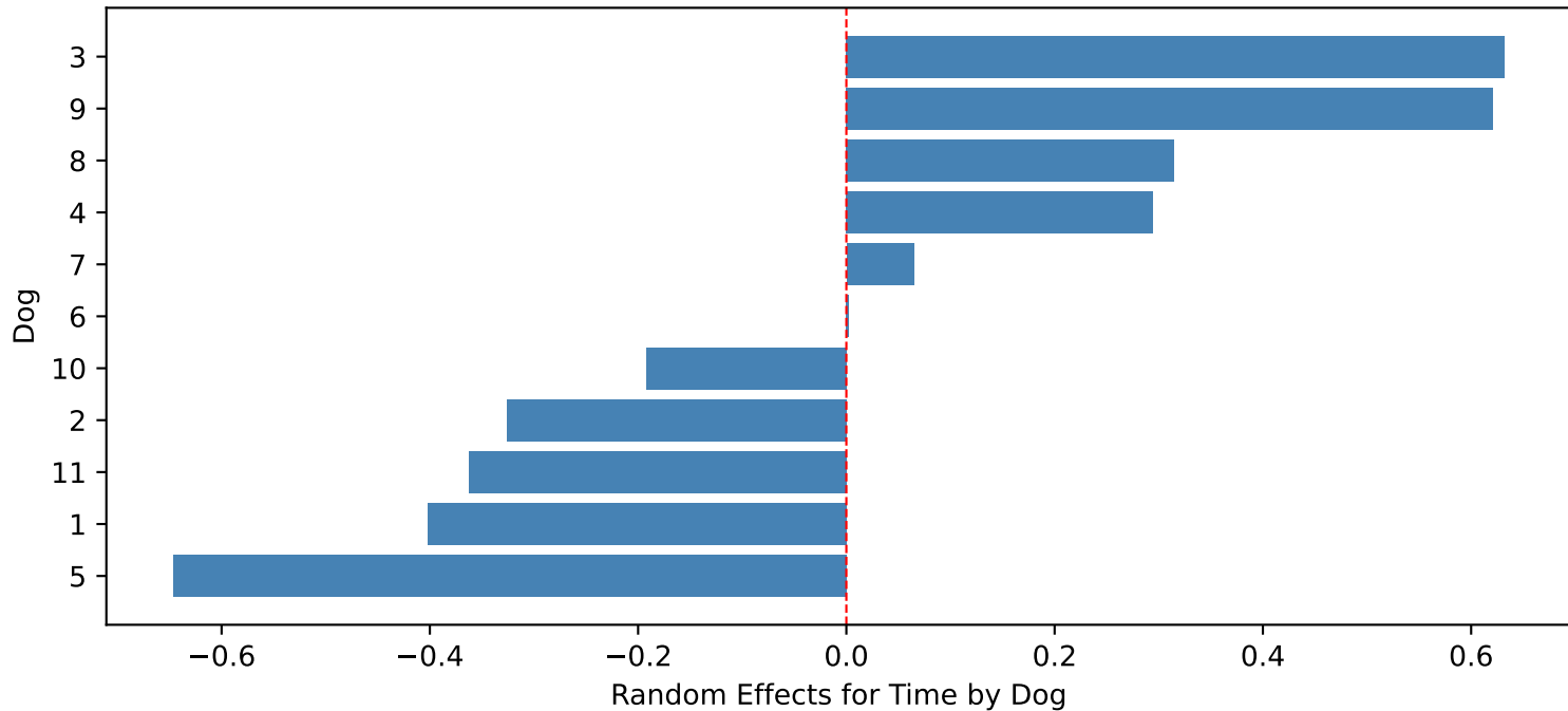
Conductivity Dog-Specific Time Slopes (BLUPs)
