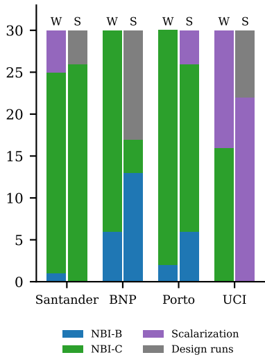
partitions where the set has the best hypervolume (of 30)
