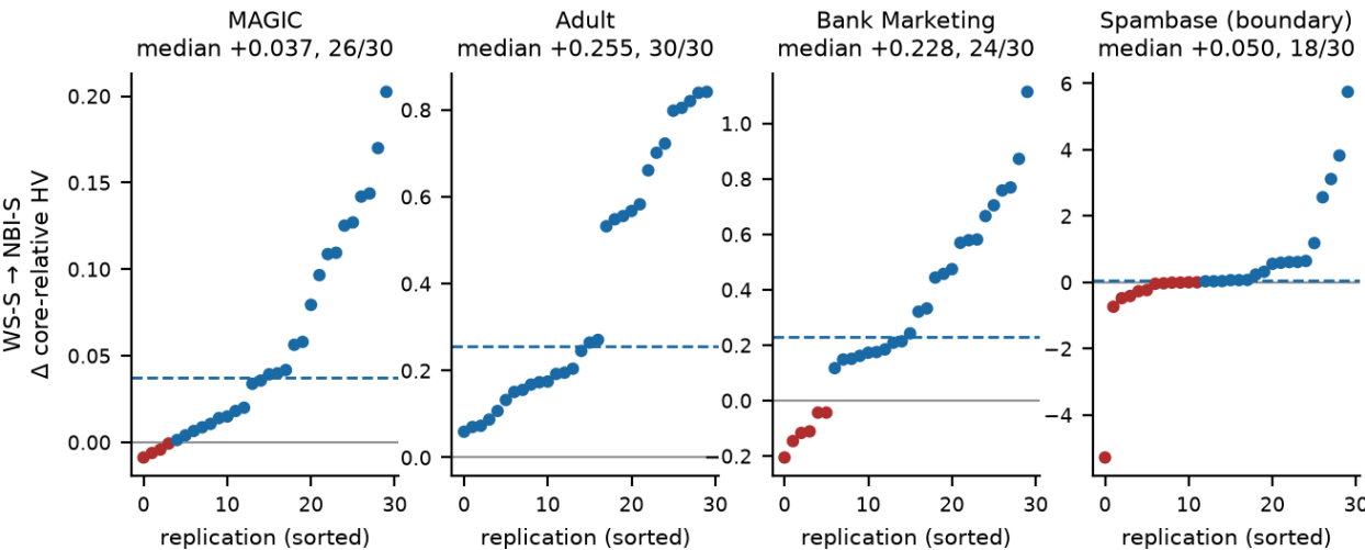
Figure 2. The geometry contrast, per replication. Paired differences in CORE-relative hypervolume ratio, NBI-S minus WS-S, sorted within each dataset, R = 30, CORE reference. Blue favours NBI-S. The dashed line is the median. Note that the vertical scales differ by dataset.
