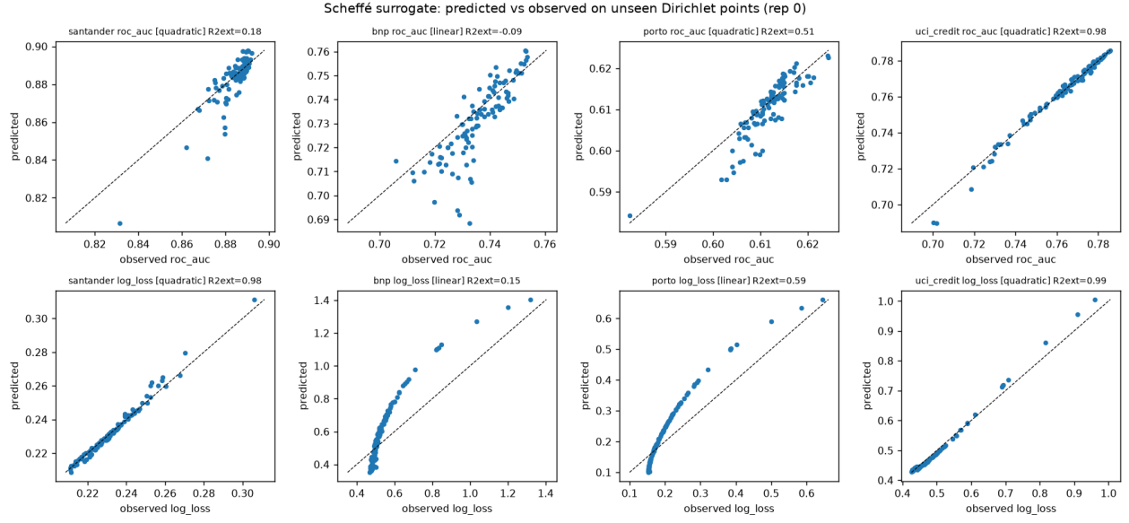
Figure S3: Predicted versus observed response on the 100 unseen compositions, all dataset–response pairs. Extends Figure 2 of the main text.
