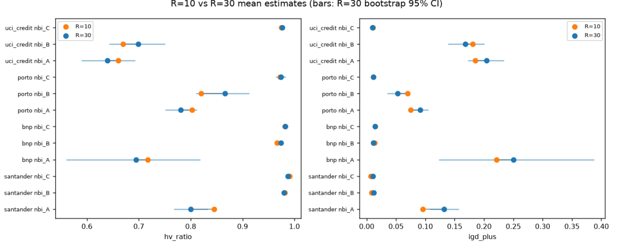
Figure S19: R = 10 against R = 30 across all metric families.
