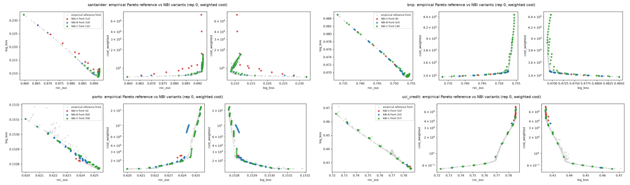
Figure S9: Revalidated fronts against the empirical reference, all four datasets. Extends Figure 3 of the main text.
