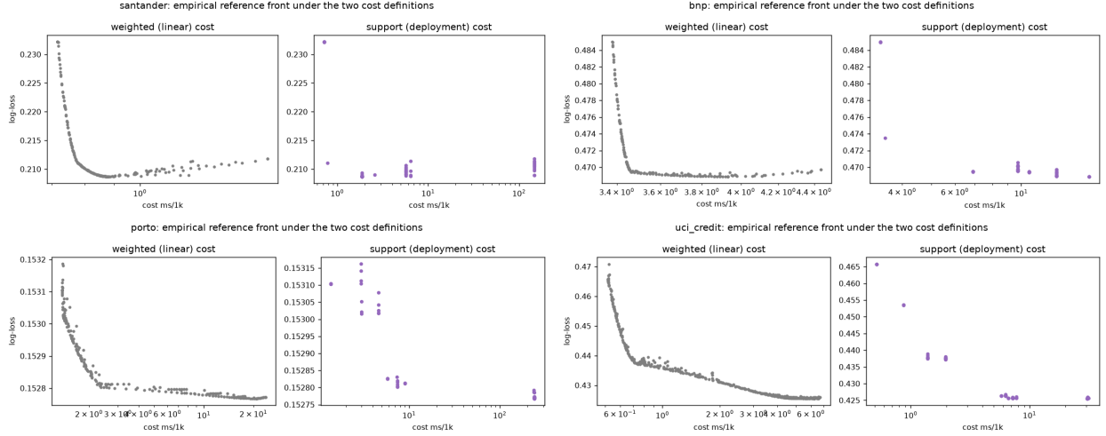
Figure S16: Weighted versus support cost, all four datasets.
