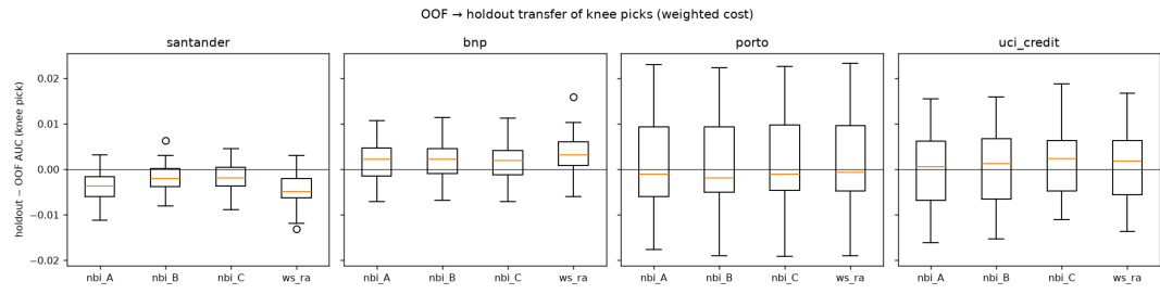
Figure S18: Holdout minus out-of-fold differences for every knee-selected solution.
