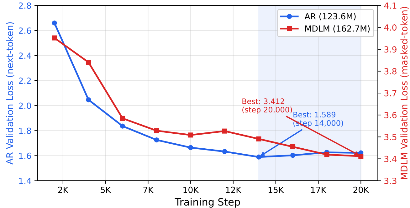
Validation Loss: AR vs. MDLM (H100, 20K steps)
