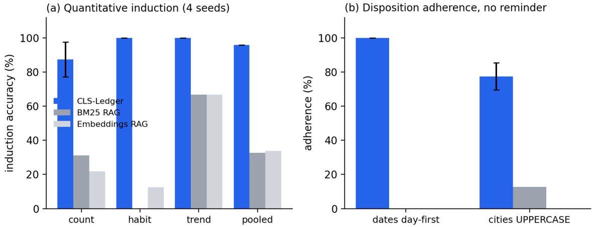
Figure 3: Figure 4: v2 capabilities, 4 seeds. (a) Induction over fact histories; (b) rule-based disposition adherence at the final exam with no reminder — a preference declaration is never lexically or semantically similar to the questions it governs, so retrieval cannot surface it.
