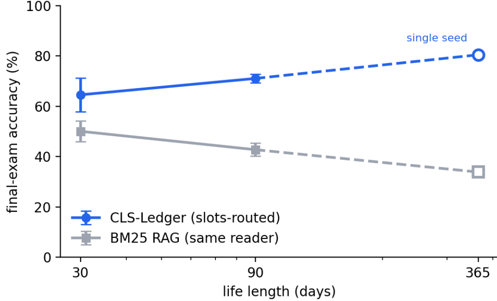
Figure 1: Accuracy vs. life length, same local reader for both systems. Error bars are sd over unseen seeds; the 365-day points are a single seed (open markers).
