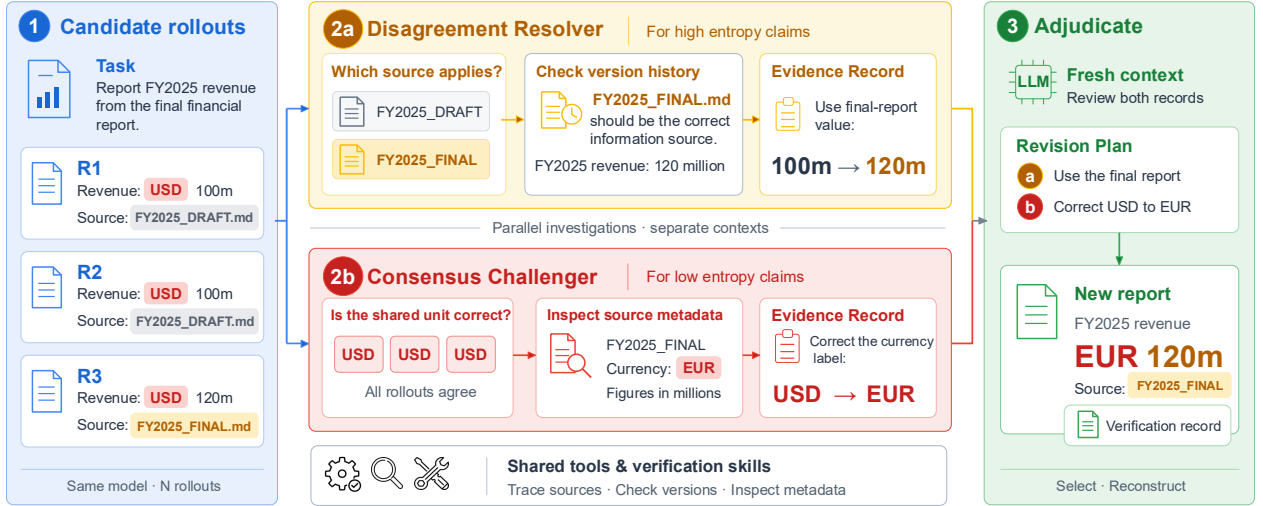
Figure 3 | VERIHARNNESS on a worked example. The task asks for FY2025 revenue from the final financial report. (1) Two rollouts cite the draft and report 100m; a third cites the final report and gives 120m, and all three label the figure USD. (2a) The resolver checks version history and establishes that the final report supersedes the draft, supporting 120m. (2b) In a separate context, the challenger checks source metadata and finds that the currency every rollout uses should be EUR. (3) Adjudication in a fresh context combines the evidence into a revision plan, and delivery produces the revised report with its verification record.
