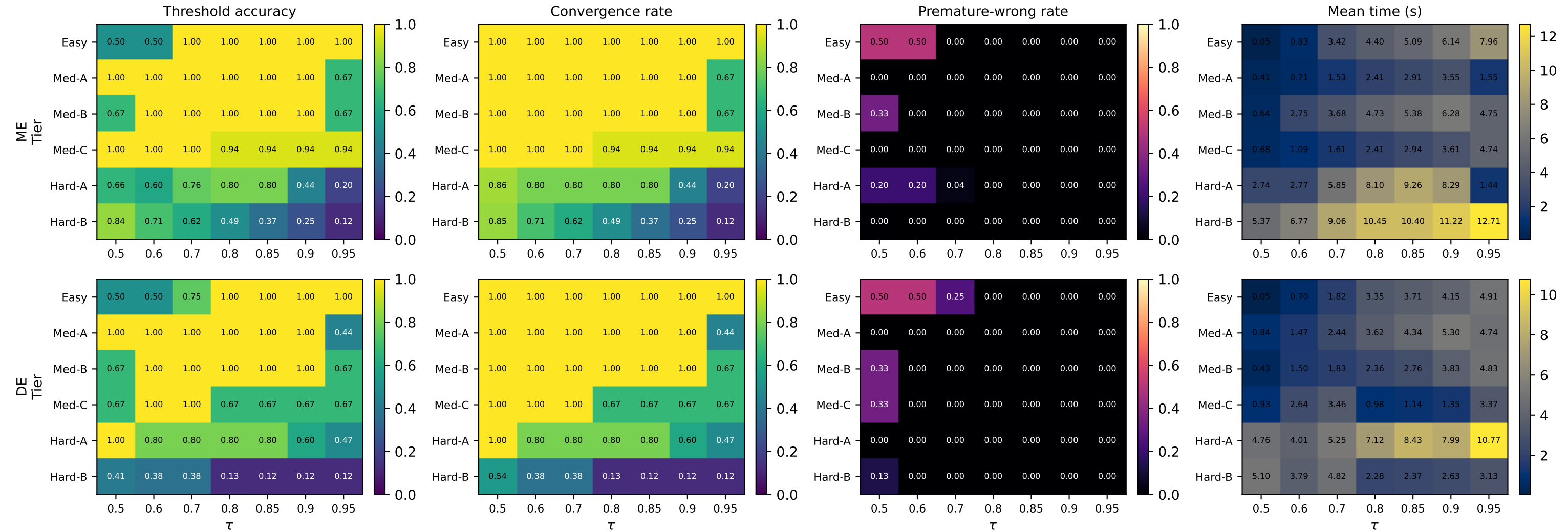
Threshold sweep: (tier x tau) heatmaps by method
