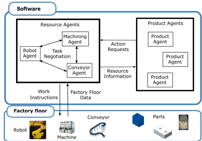
Fig. 1. The interactions between product agents, resource agents, and the factory floor in a multi-agent architecture.
