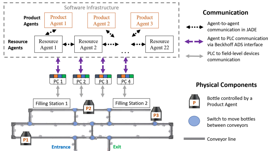
Fig. 3. The setup and infrastructure for the myJoghurt system at the Institute of Automation and Information Systems, Technical University of Munich.
