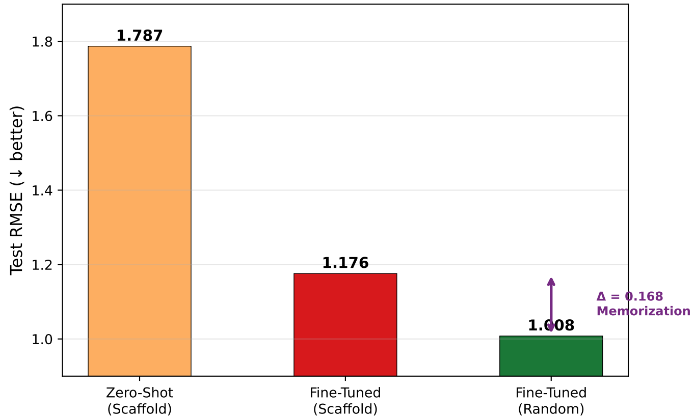
PSICHIC: Scaffold → Random Split
