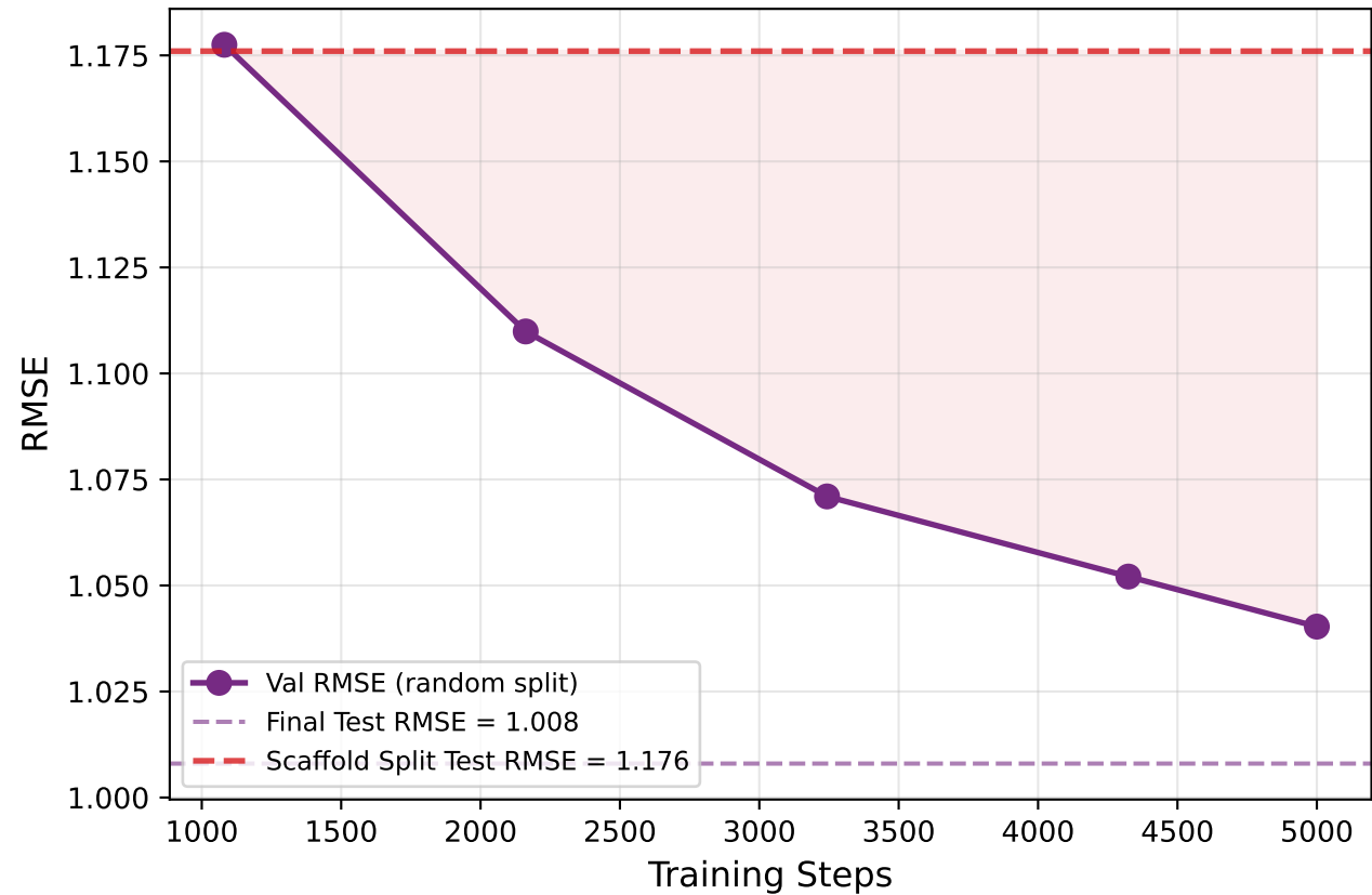
PSICHIC Fine-tuned on Random Split Val RMSE Progress
