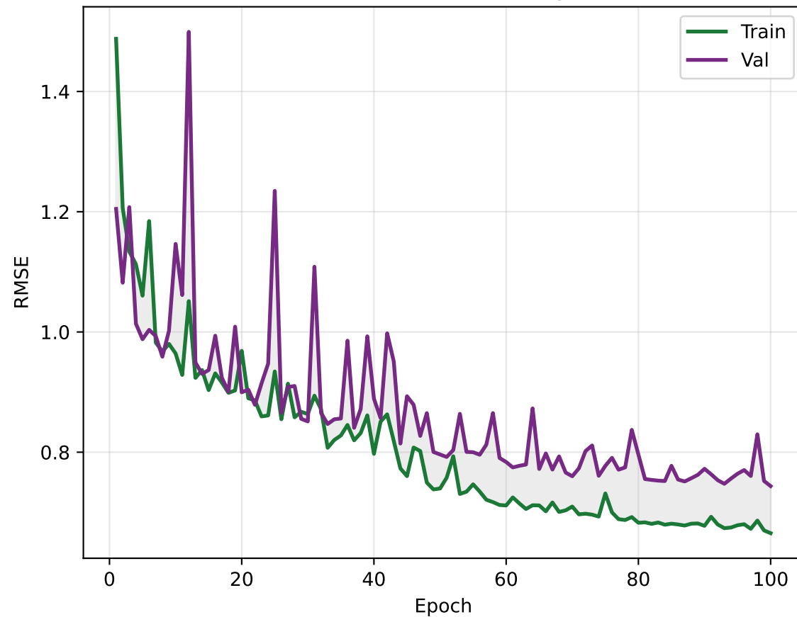
MLP shallow [256], 1 layer
