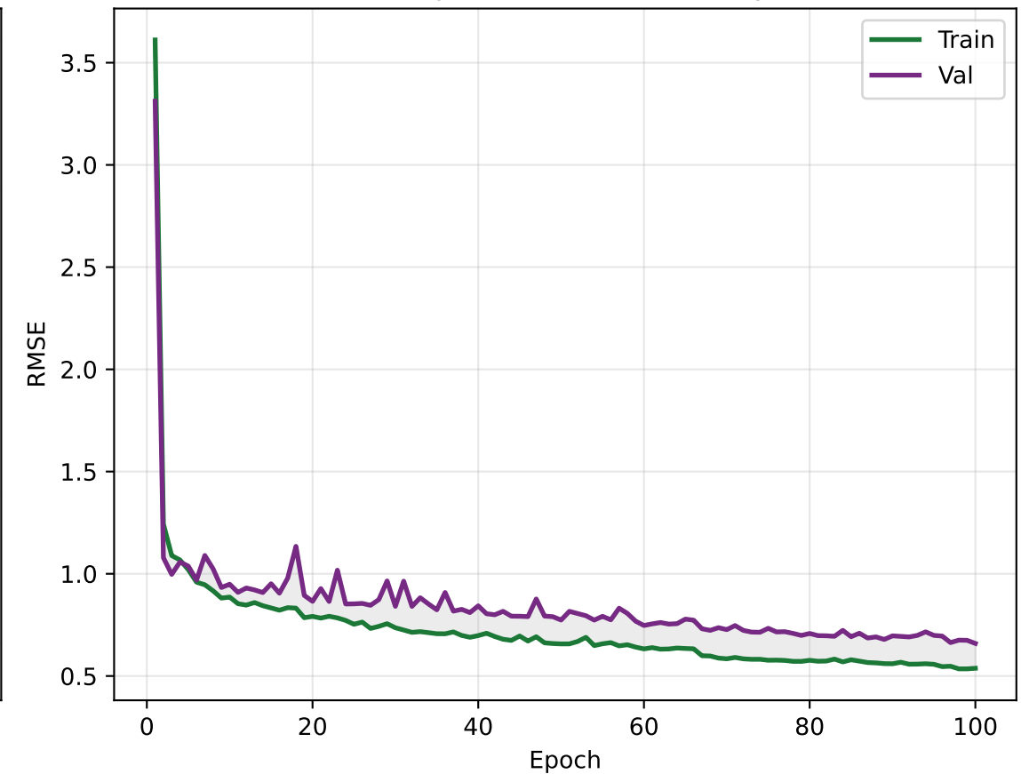
MLP deep [512, 256, 128], 3 layers
