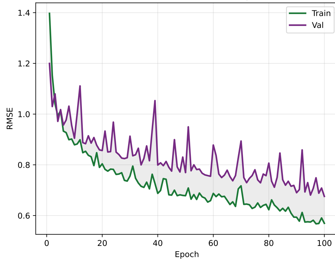
MLP medium [512, 256], 2 layers
