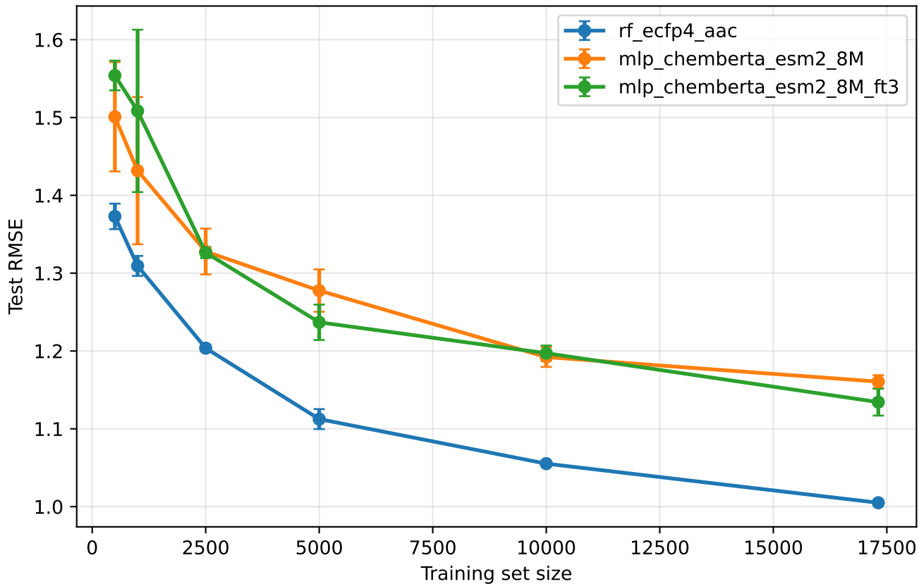
E201: Learning Curves
