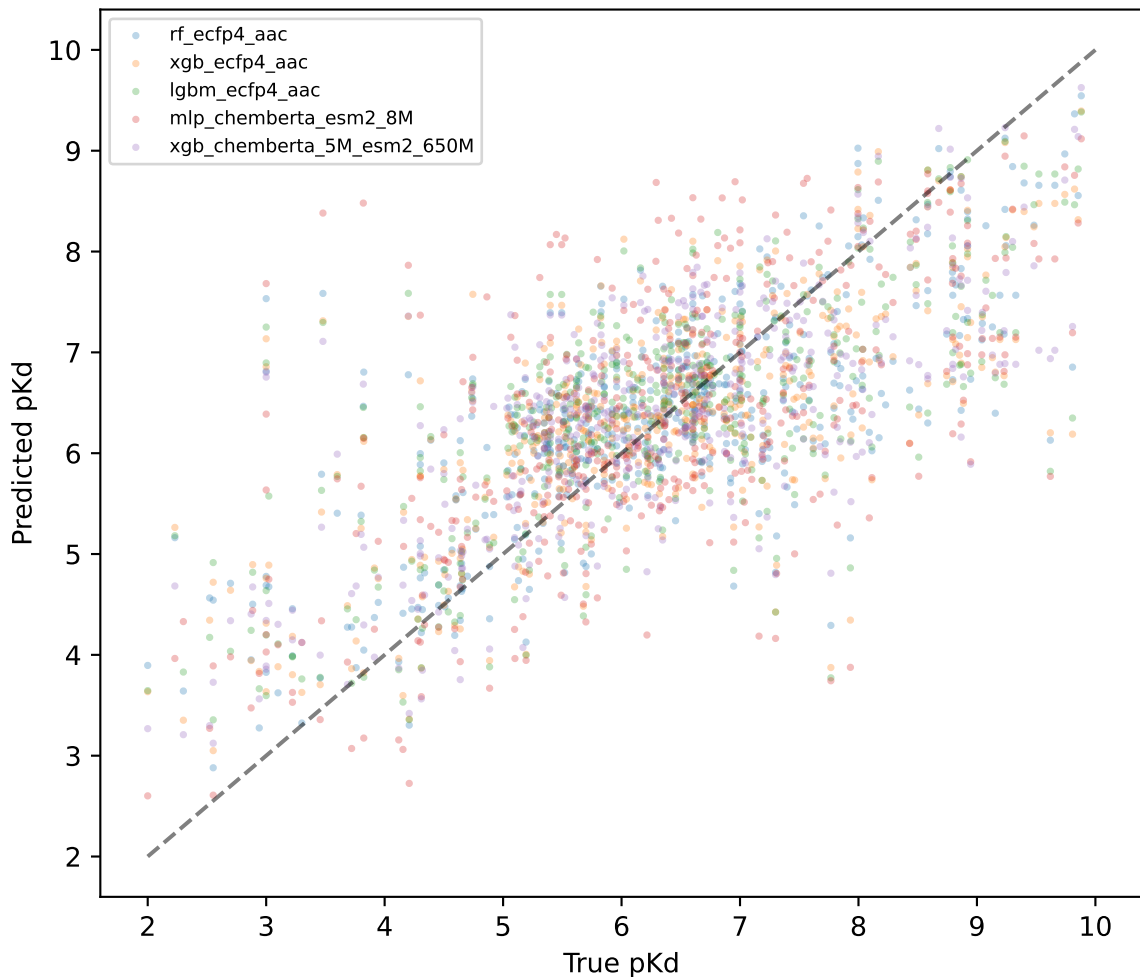
E302: Predicted vs True
