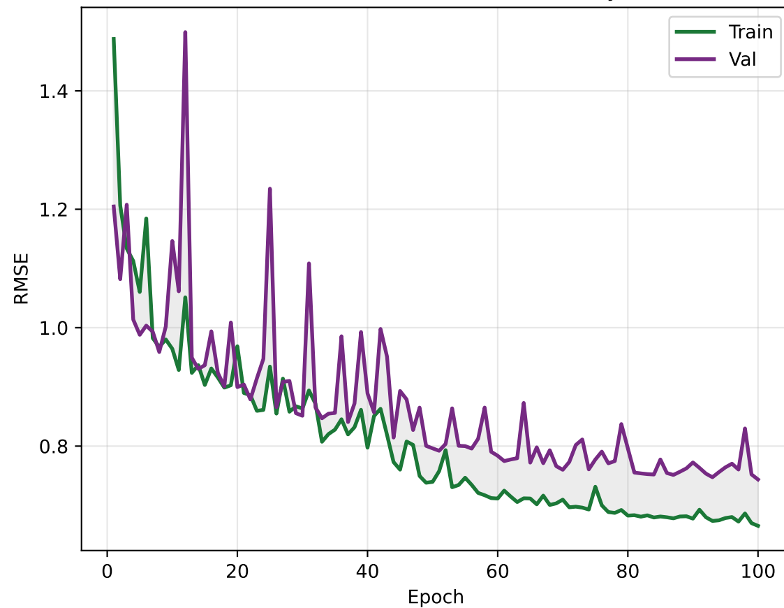
MLP shallow [[512, 256, 128]] , 3 layers
