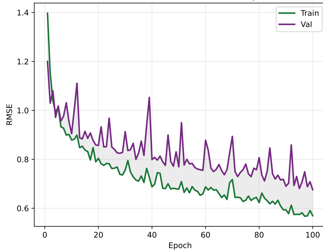
MLP medium [[512, 256, 128]] , 3 layers
