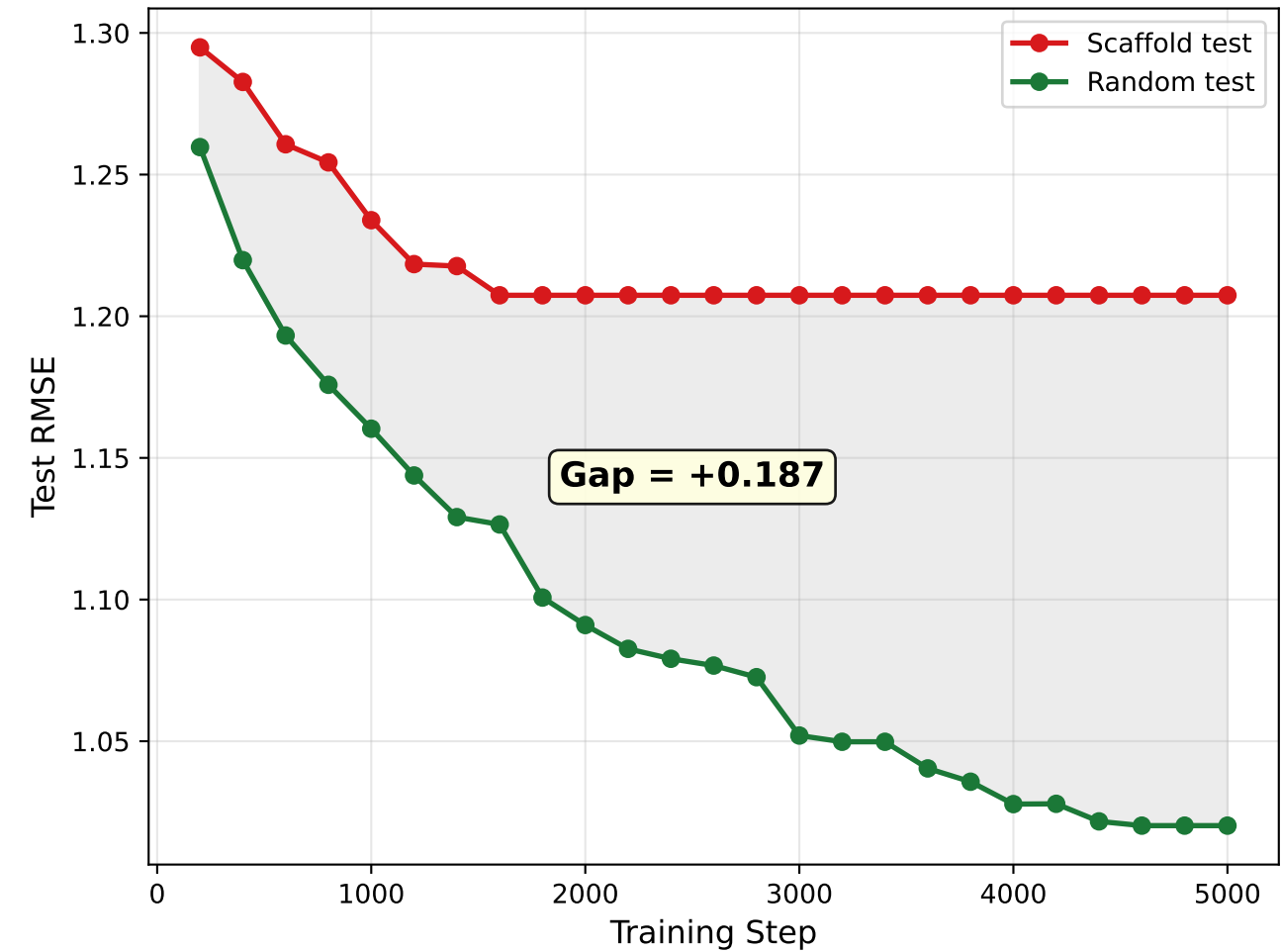
Memorization Gap: Scaffold vs Random
