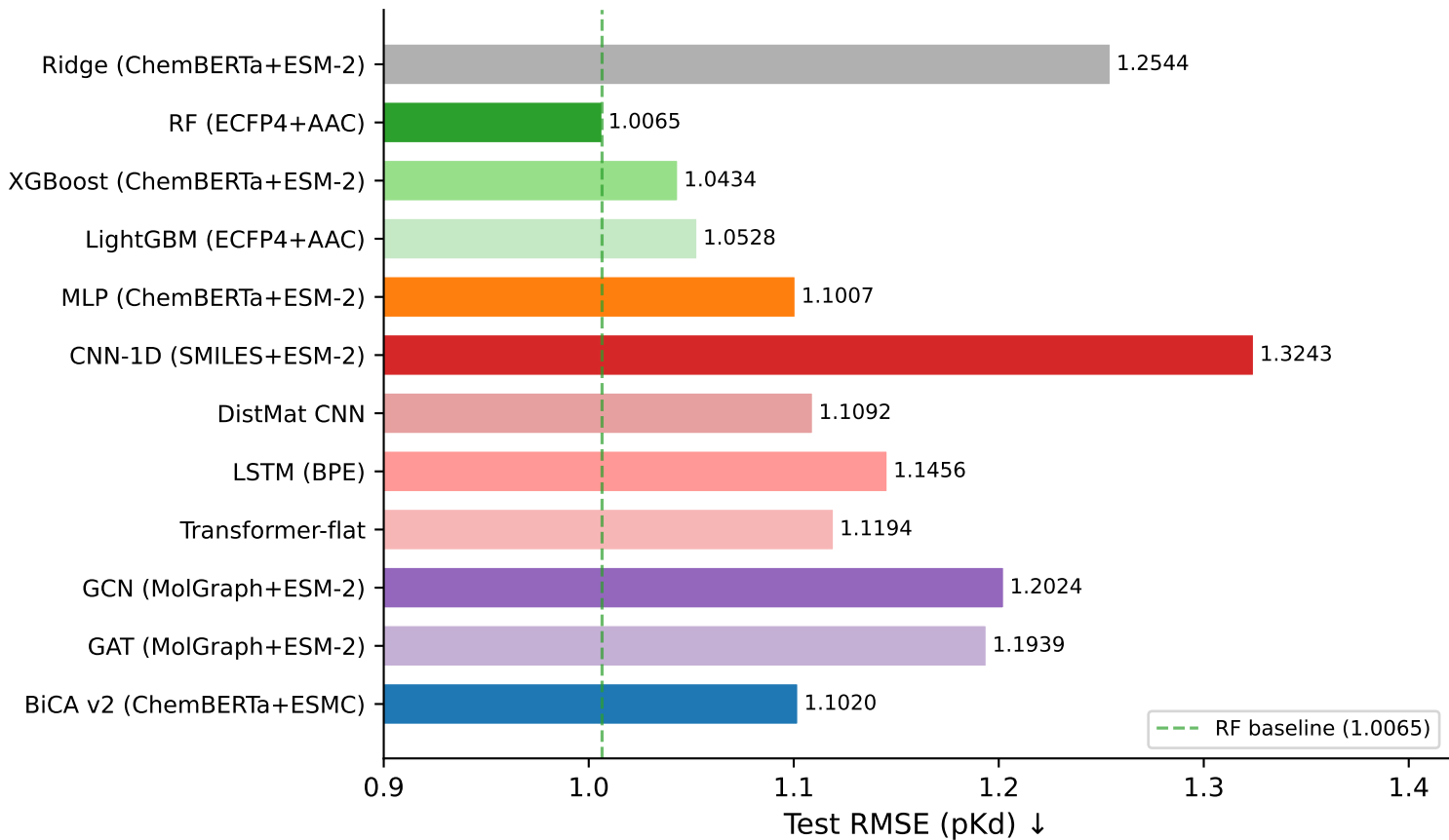
Best model per family — BindingDB_filtered scaffold split
