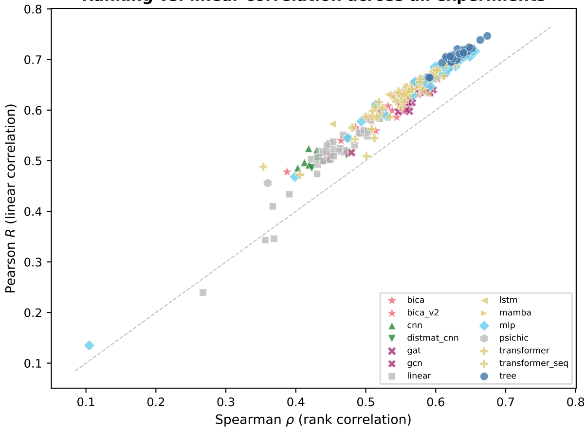
Ranking vs. linear correlation across all experiments
