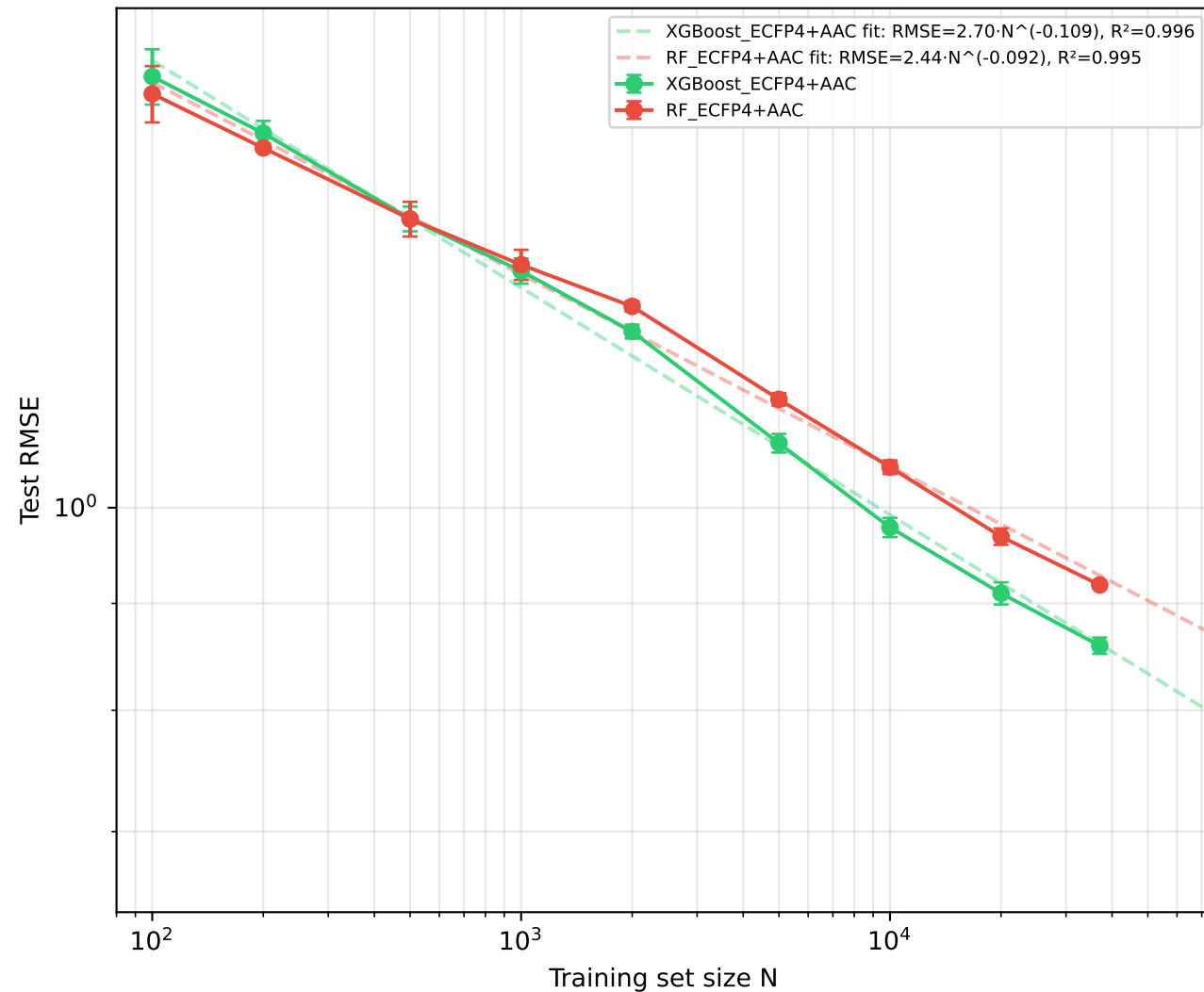
Random Split — Learning Curves
