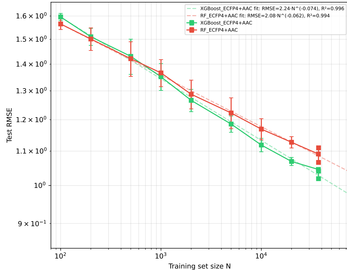
Scaffold Split — Learning Curves
